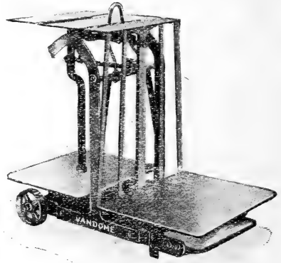
No. 155. Wrought Iron Machines.
