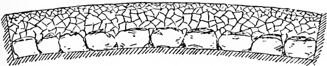
Fig. 86.—A Telford road.
