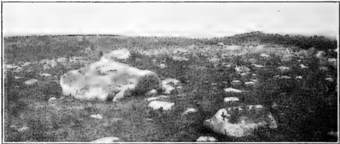
A glacial soil. The large rocks are boulders, commonly found in soils formed by glaciers.
