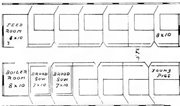
40. GROUND PLAN OF PIGGERY.
