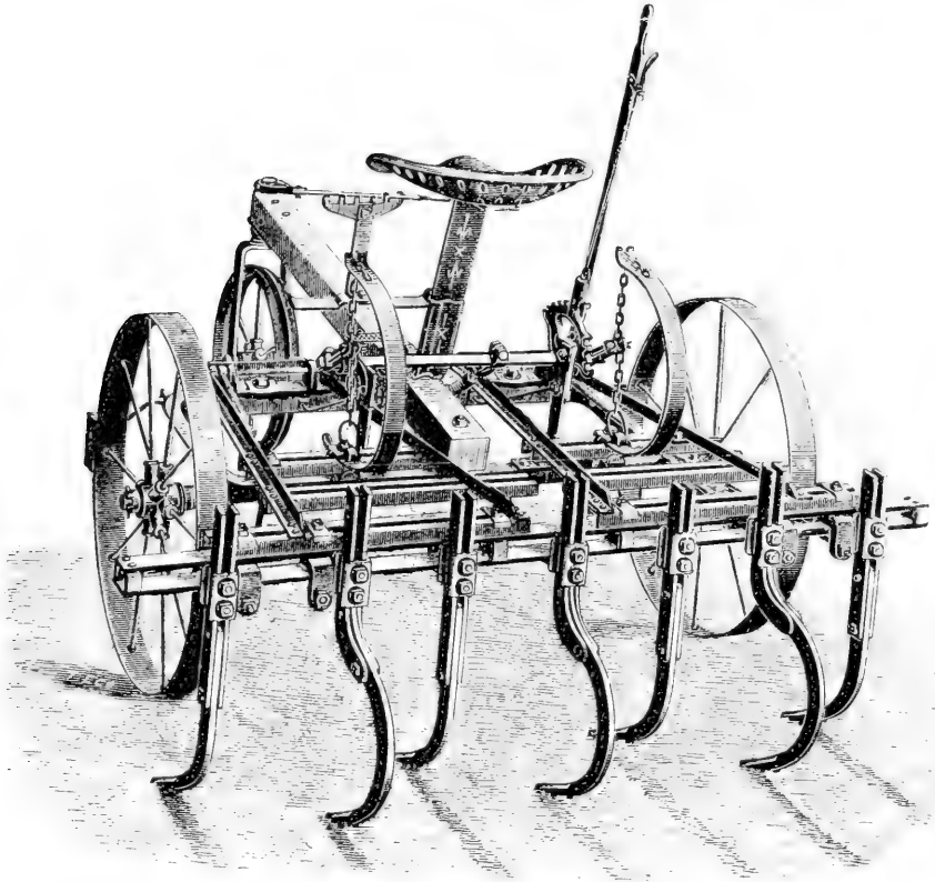
1. FOUR-HORSE SUBSOILER.
