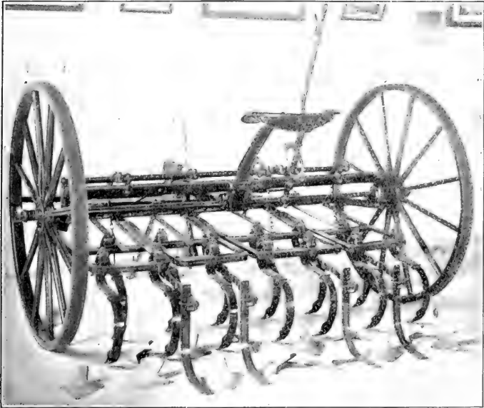
47. STRING TOOTH CULTIVATOR
