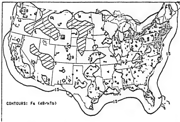
Figure 13. Nighttime 45 MHz airborne man-made radio noise map of the continental United States for an altitude of 30 thousand feet.
