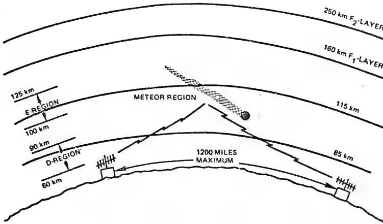
Figure 1. Meteor Burst Communication System.
