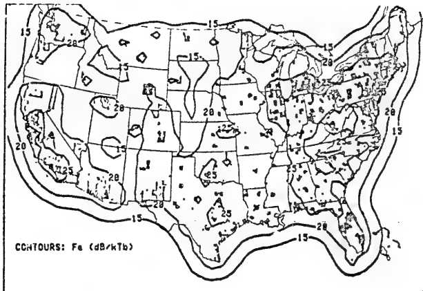
Figure 15. Daytime 30 MHz airborne man-made radio noise map of the continental United States for an altitude of 30 thousand feet.
