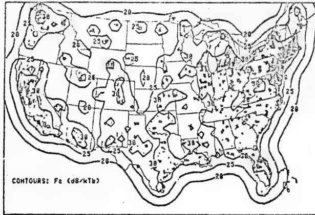
Figure 16. Daytime 70 MHz airborne man-made radio noise map of the continental United States for an altitude of 30 thousand feet.
