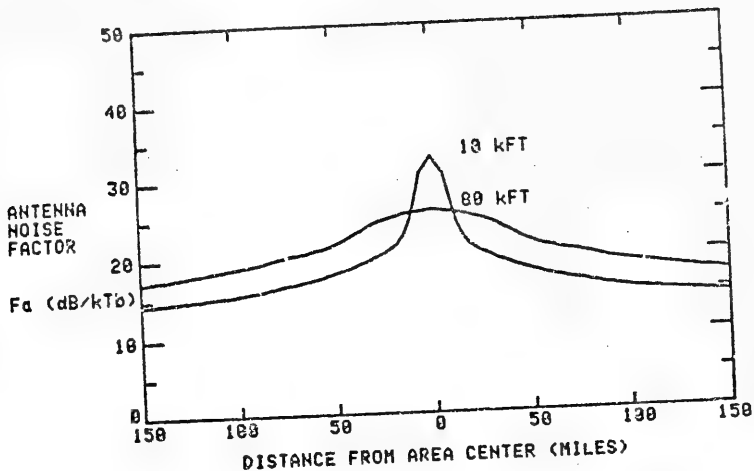
Figure 8. Daytime 45 MHz man-made radio noise model for altitudes of 10 and 80 thousand feet above a business area. Radio noise power, F_a (dB/kTb), is plotted as a function of distance in miles from the city center.
