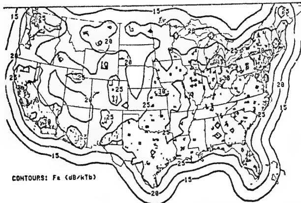
Figure 11. Daytime 45 MHz airborne man-made radio noise map of the continental United States for an altitude of 20 thousand feet.
