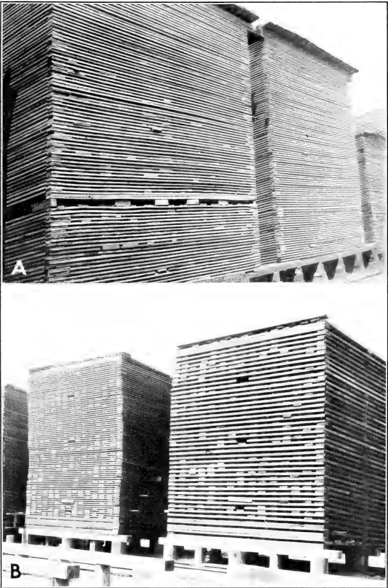
A.—Eight-inch horizontal opening in lower part of pile B.—A common method of single-length roof construction
