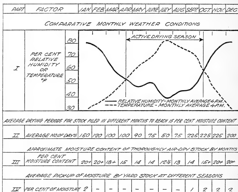
FIG. 7.—Graphic air-seasoning chart for the Inland Empire
