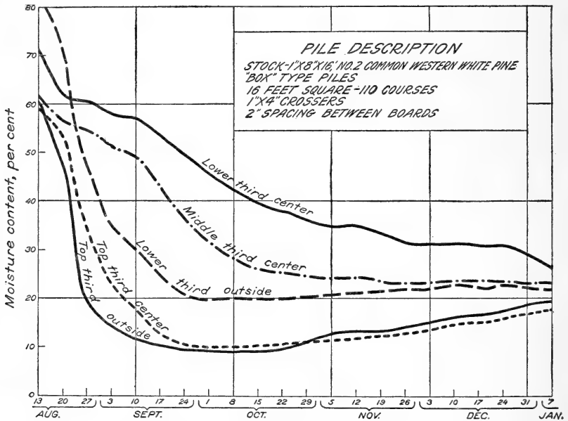
FIG. 1.—Comparative rate of drying in different parts of typical lumber pile
