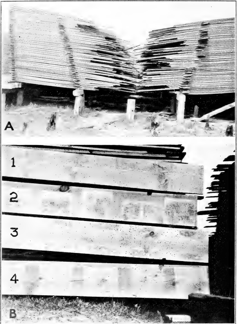
A.—The random-length type of pile B.—Common pile stock crossers 1×12 inches, 16 feet long. Season check shows in Nos. 1 and 4. Crosser-stain has developed in Nos. 2 and 3
