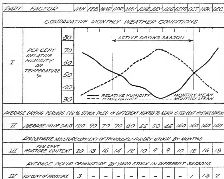
Fig. 8.—Graphic air-seasoning chart for the California pine region
