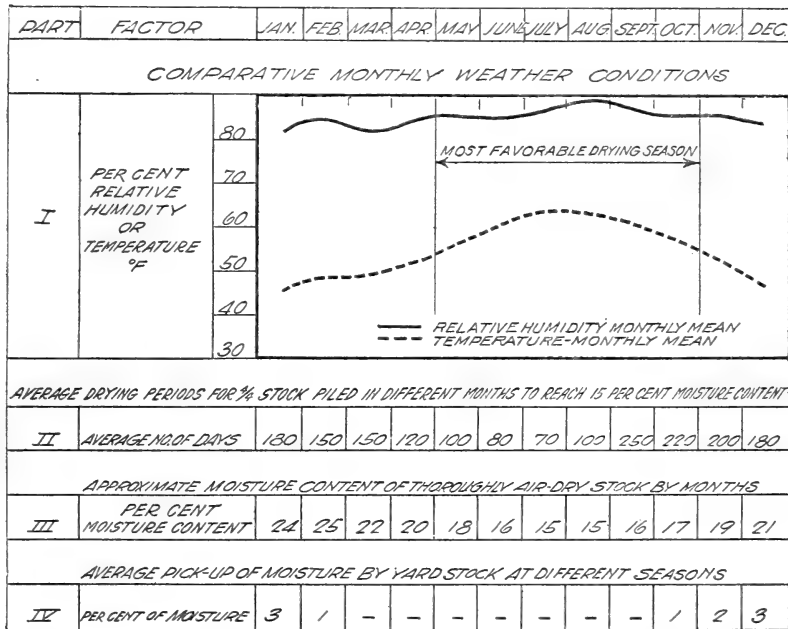
FIG. 9.—Graphic air-seasoning chart for the redwood region
