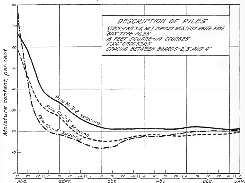
FIG. 5.—Comparative "pile average" drying rates for stock piled with different spacing between boards
