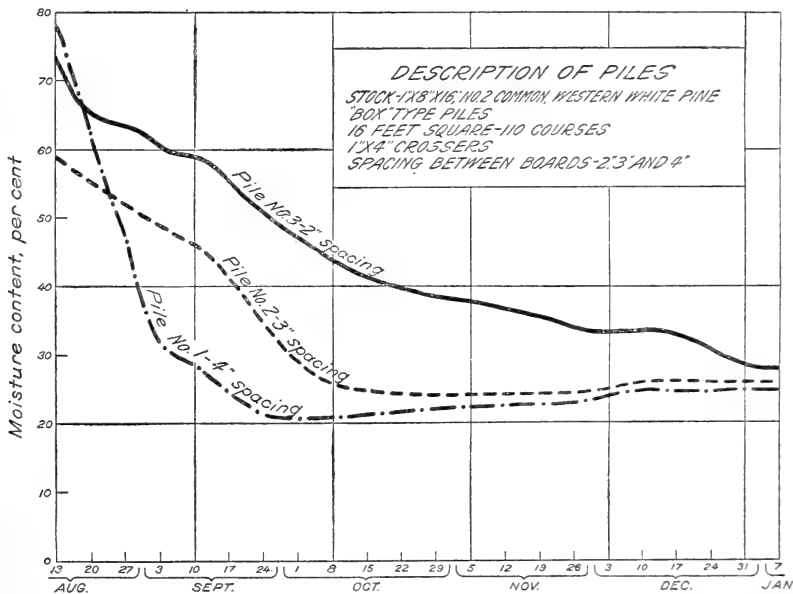
FIG. 6.—Comparative drying rates in lower third of pile for stock piled with different spacing between boards
