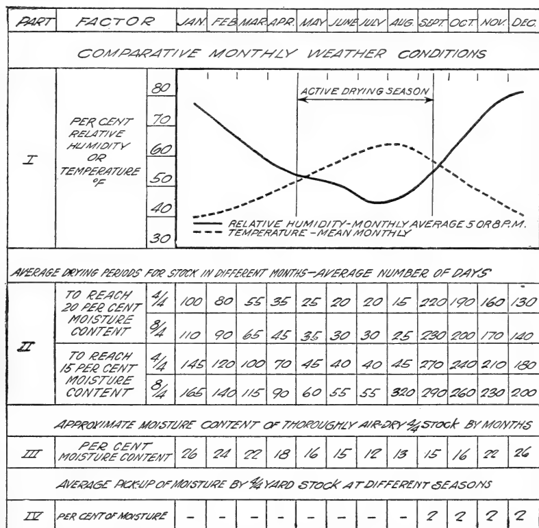
Fig. 10.—Graphic air-seasoning chart for the Douglas fir region
