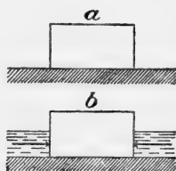
FIG. 104. DIAGRAMS ILLUSTRATING NON-FLOTATION THEORY OF TIDAL GLACIERS.
