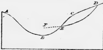
FIG. 58. DIAGRAM ILLUSTRATING DISCORDANCE OF HANGING VALLEYS.
