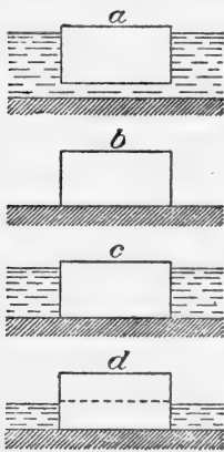
FIG. 103. DIAGRAMS ILLUSTRATING FLOTATION THEORY OF TIDAL GLACIERS.
