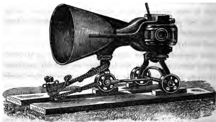
FIG. 6.—Breech-loading Fog-signal Gun, with Bell Mouth, 1 proposed by Major Maitland, R.A., Assistant Superintendent.
