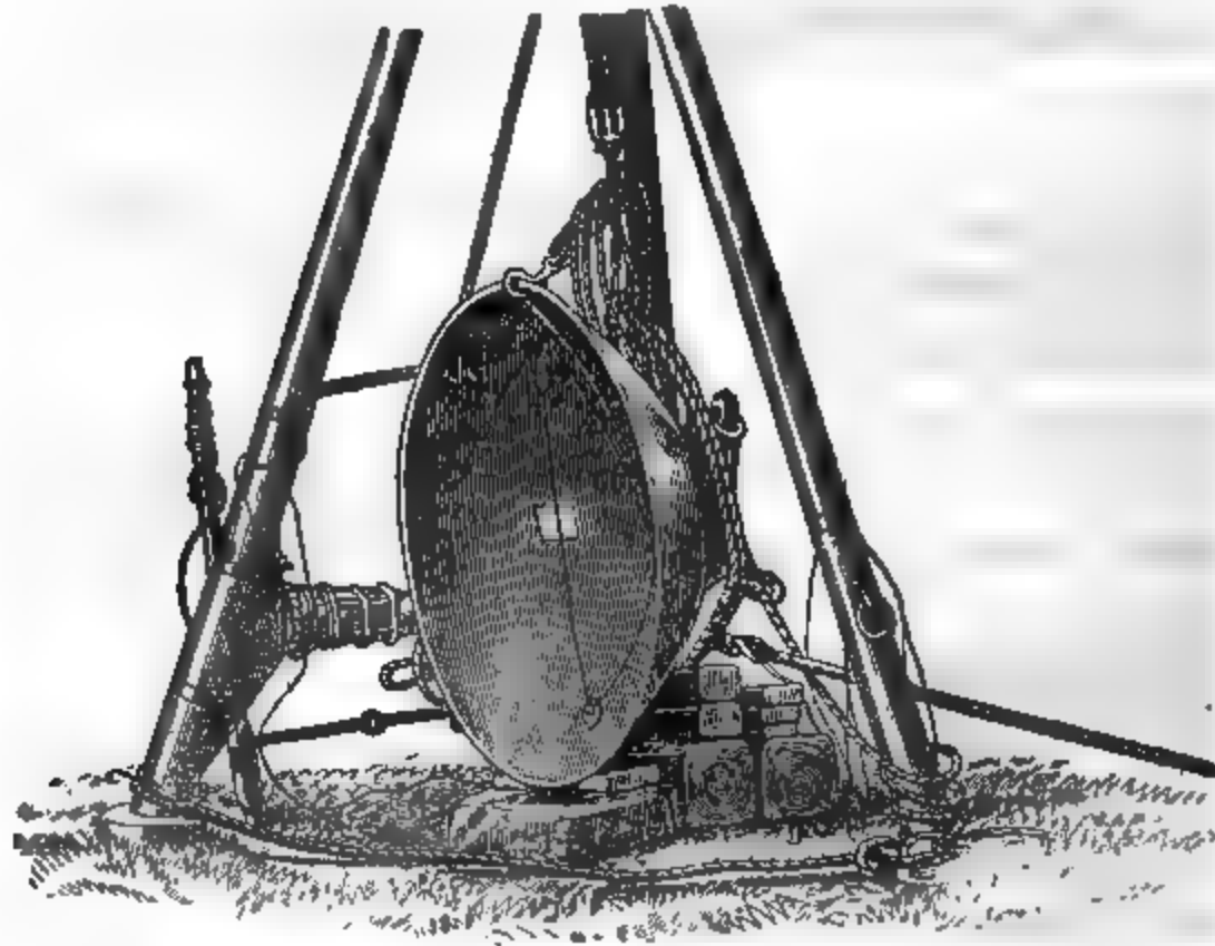
FIG. 8.—Gun-cotton Slab ( 1\frac{1}{2} lb.) Detonated in the Focus of a Cast-iron Reflector
