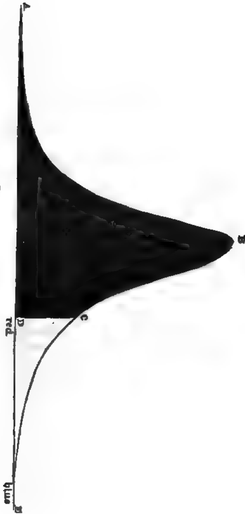
FIG. 1.—Spectrum of Incandescent Light.
