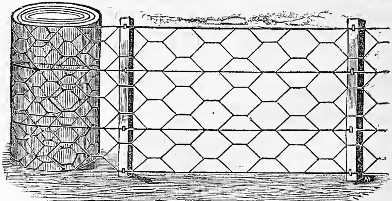
IMPROVED WIRE FENCE.
