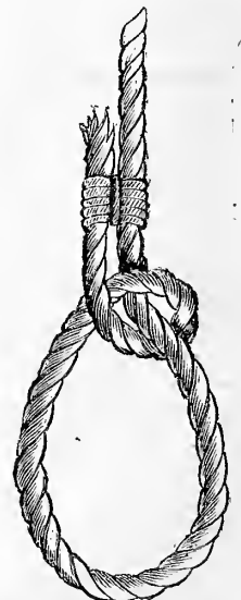
Fig. 6.—HALF HITCH SEIZED FOR EYE.
