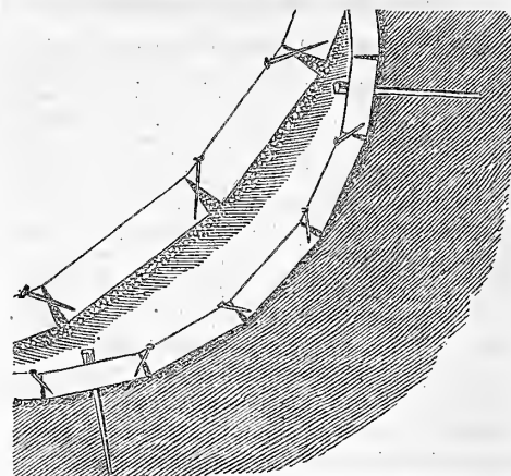
Fig. 2.—WOODEN CURBING.
