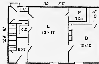
GROUND PLAN.
