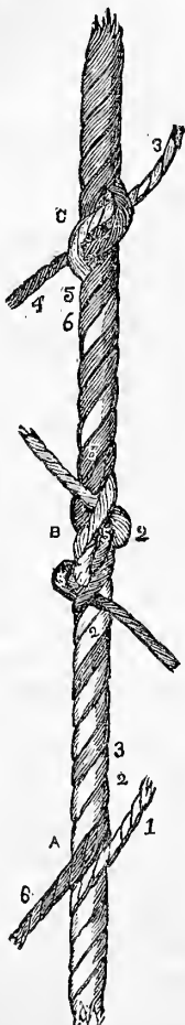
Fig. 4. LONG SPLICE.
