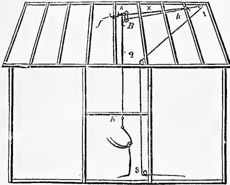
Fig. 1.—HAY FORK ATTACHMENT IN PLACE.
