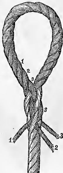
Fig. 2. SPLICED EYE.
