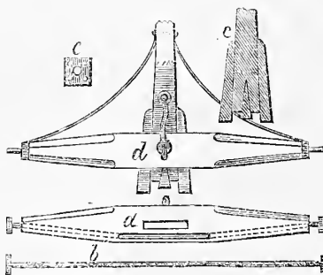
Fig. 6.—ROLLER, ETC.
