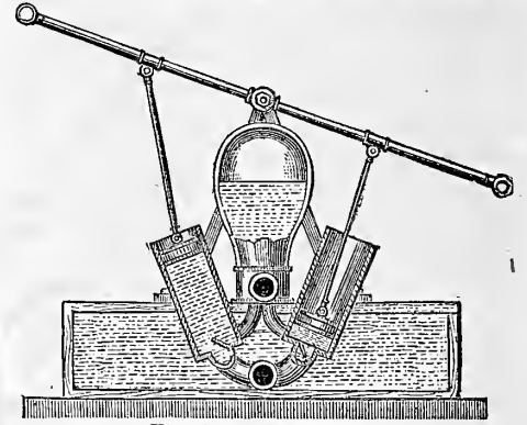
Fig. 2.—FIRE ENGINE.
