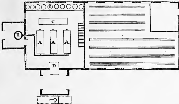
Fig. 2.—PLAN OF A CHEESE FACTORY.
