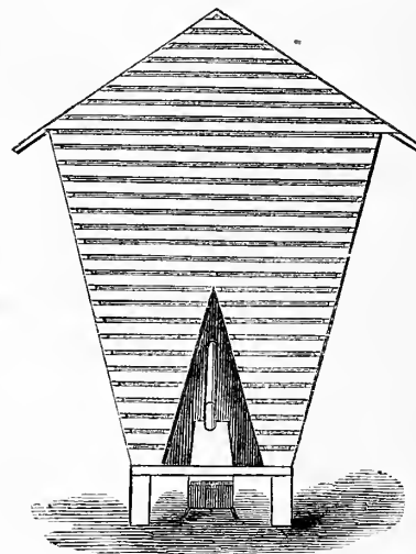
CRIB ARRANGED AS A KILN.
