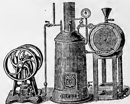
Fig. 2.—ENGINE, BOILER, AND WATER-TANK.
