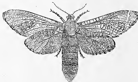
Fig. 4.—FEMALE MOTH.
