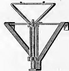
Fig. 1.—SEAT SPRING.
