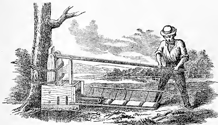
Fig. 1.—TILE-MAKING MACHINE.
