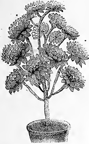
Fig. 1.—TREE HOUSE-LEEK.
