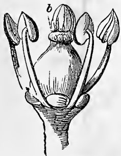
Fig. 1.—GRAPE.
