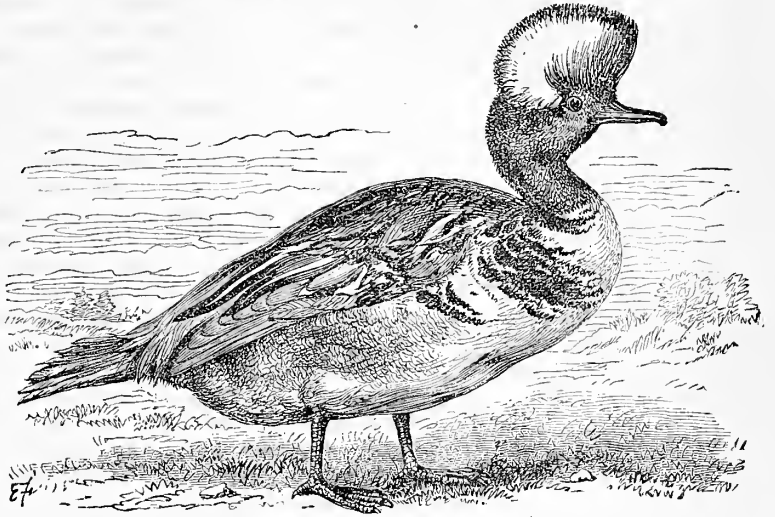
Fig. 2.—HOODED MERGANSER.
