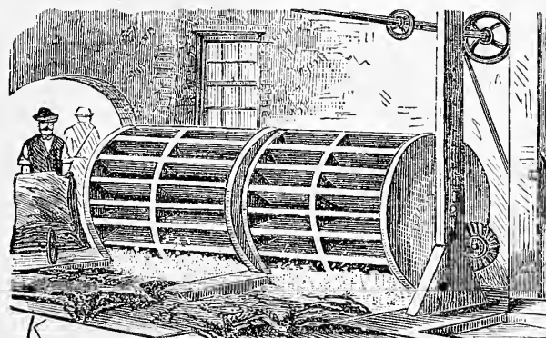
Fig. 6.—BATHING WHEELS.
