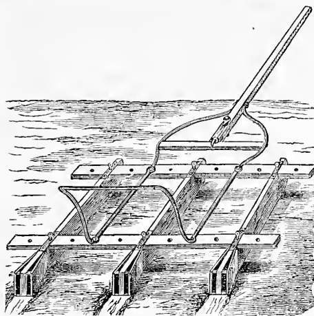
A CORN-MARKER.
