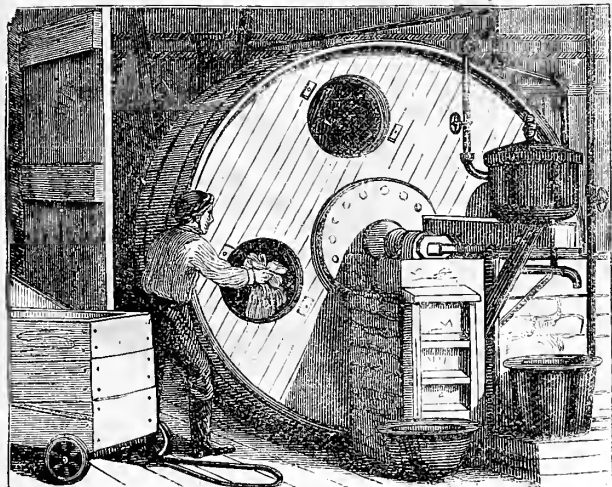
Fig. 1.—WASHING MACHINE.
