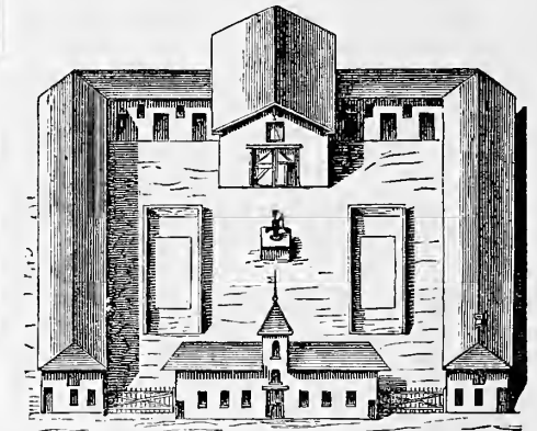
Fig. 2.—ELEVATION OF BUILDINGS.
