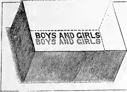
Fig. 1.—DOUBLE REFRACTION.
