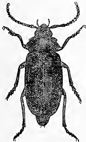
Fig. 2.—OAK-BORER BEETLE.
