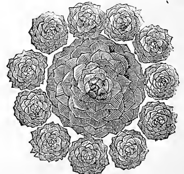
Fig. 4.—HAIRY HOUSE-LEEK.
