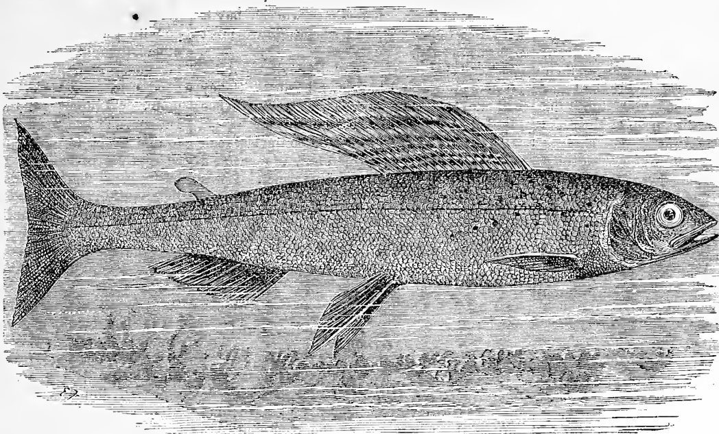
THE GRAYLING.
