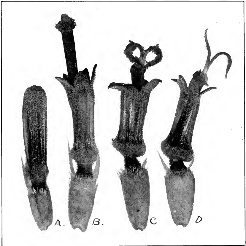
FIG. 2.—DISK FLORETS OF HELIANTHUS (enlarged five diameters).
