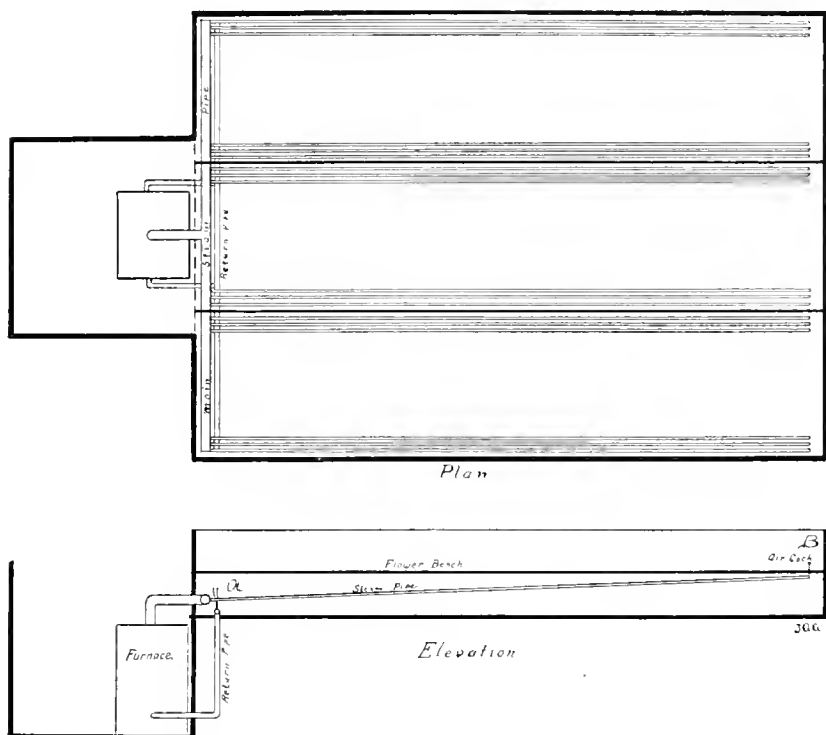
THE SINGLE PIPE SYSTEM OF HEATING GREENHOUSES AS USED BY MR. THOS. FRANKS, CHAMPAIGN, ILL
