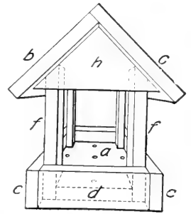
FIG. 10.—Nest shelter.
