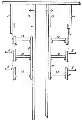
FIG. 35.—Longitudinal vertical section of martin house; lowered, and doors closed.
