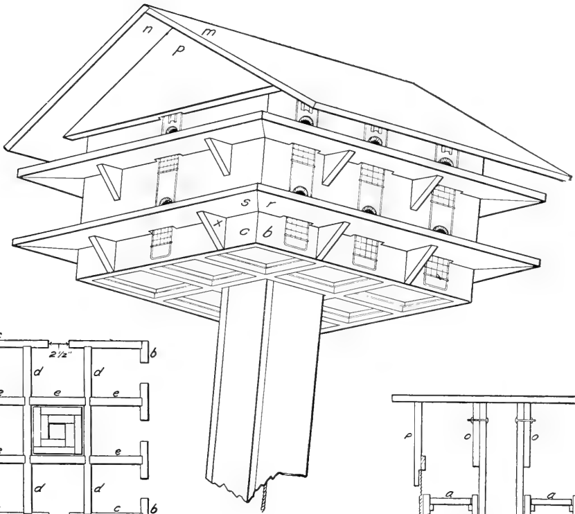
FIG. 32.—Martin house.
