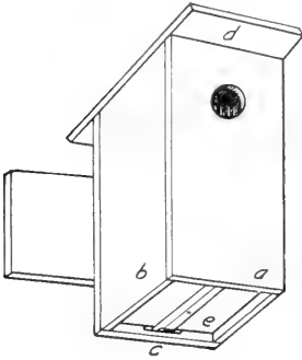
FIG. 19.—Style of house suitable for sparrow hawks, screech owls, bluebirds and wrens. Designed to be placed in trees. Bottom can be removed by turning button.
