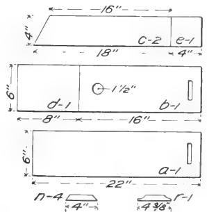
FIG. 27 Lumber diagrams of house shown in figure 25, suitable for downy woodpecker. By reducing size of entrance it becomes right for titmice and nuthatches. Thickness of boards \frac{3}{4} inch.
