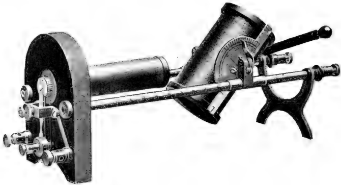
FIGURE 1.—The inductorium.
