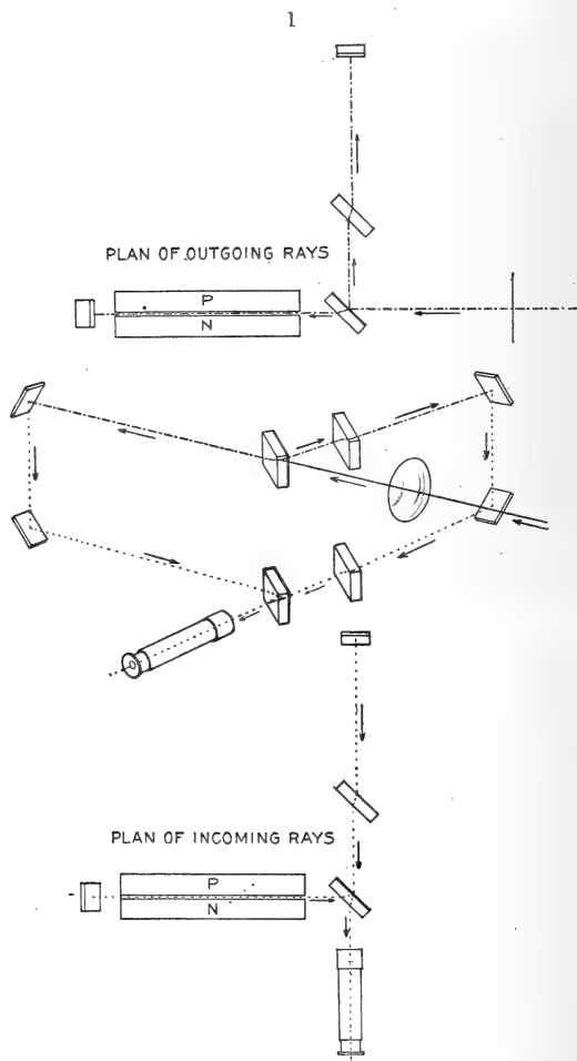
FIG. 1. Plan of Refractometer.
