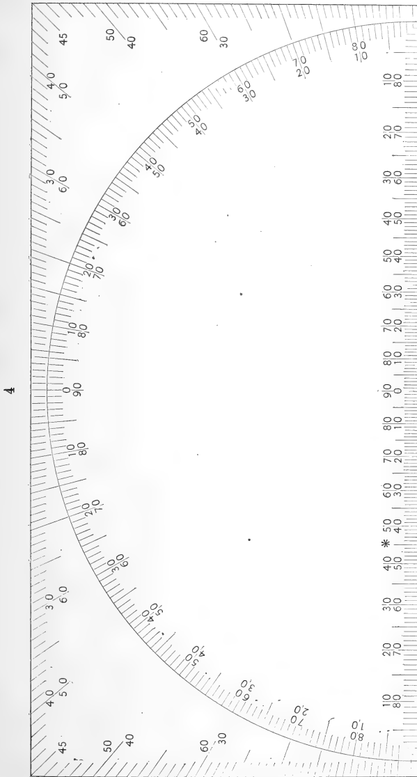
PROTRACTOR NO. 1, FOR PLOTTING STEREOGRAPHIC PROJECTIONS.
