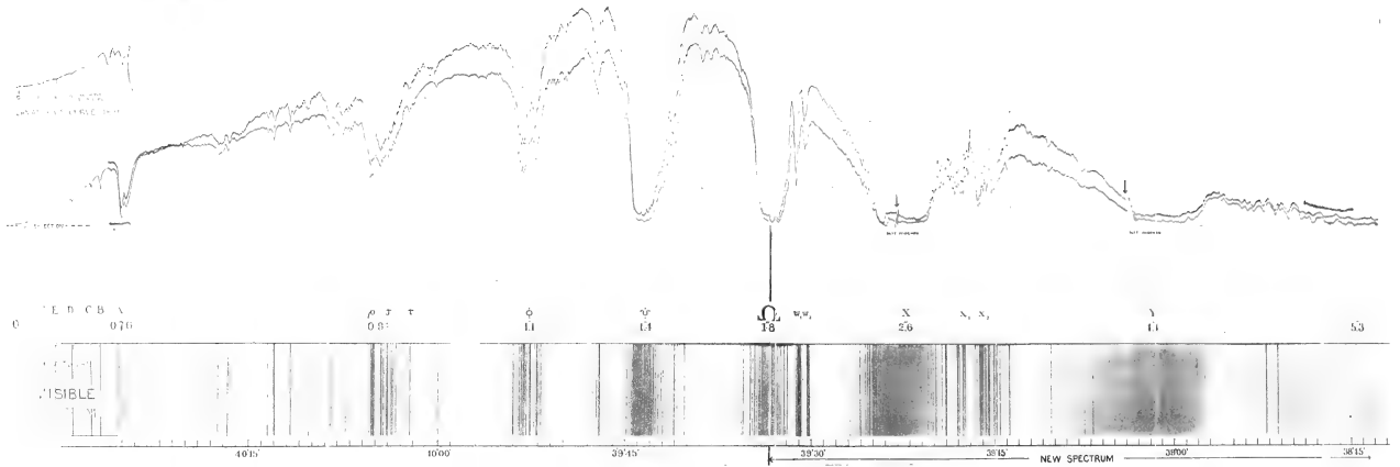
Reduction from Large Map of the Infra-red Solar Spectrum of a 60 Rock-Salt Prism. Energy Curves and Line Spectrum from Holographs of 1898 Observations of S. P. Langley with the assistance of C. G. Abbot.
