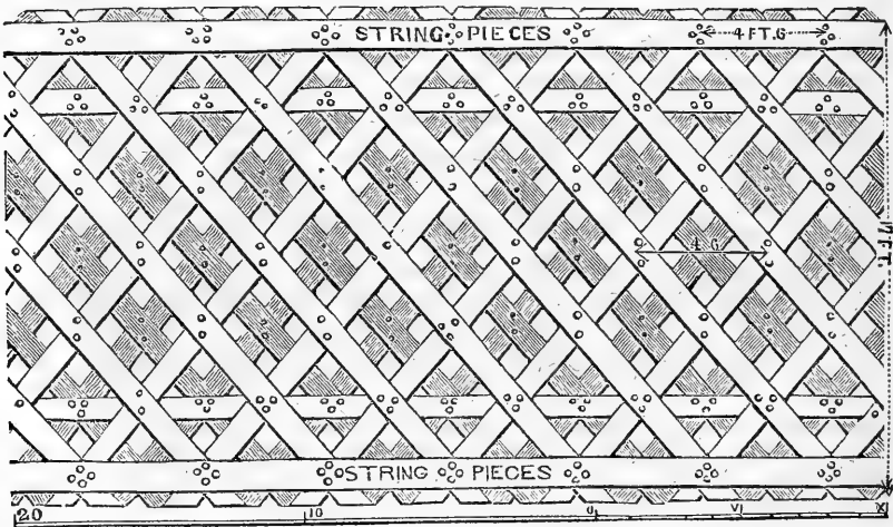
No. 2. The side elevation of a truss, to the same scale. The height of a truss may be greater or less, by any number of half diamonds, or by a change of the angle of the truss-braces.
