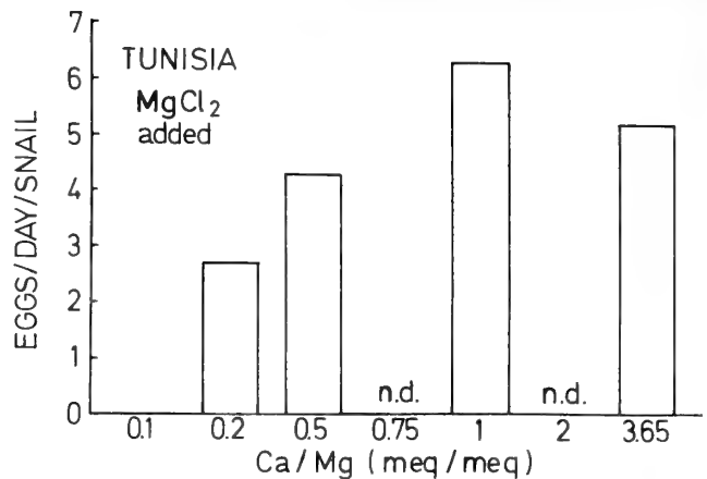
Fig. 2. Egg laying rates in Tunisian Bulinus truncatus in artificial media. One replicate. Ratios varied by addition of \text{MgCl}_2 \cdot 6 \text{H}_2\text{O} to SFW 100 (0.1/1 only in the replicate). Total chlorides see figure 1. Mean values of counts over three or (replicate) four weeks, 4 x 4 snails, 8 to 9 mm high, in 100 ml medium each.
