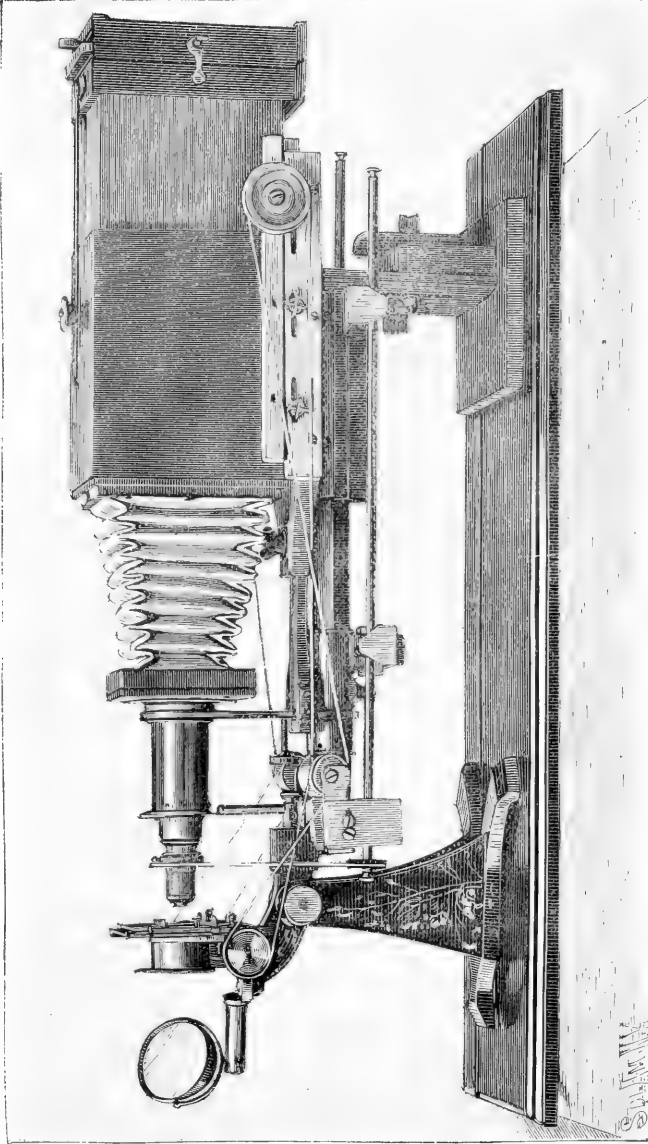
PHOTO-MICROGRAPHIC APPARATUS
