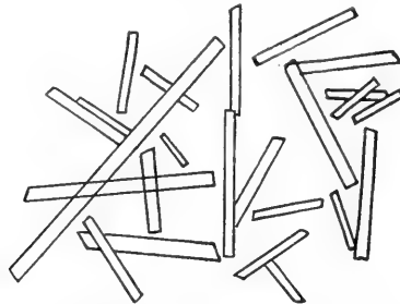
Crystals from "Vaseline-Cocaine," 1 in 20. ( \frac{1}{4} inch objective.)
