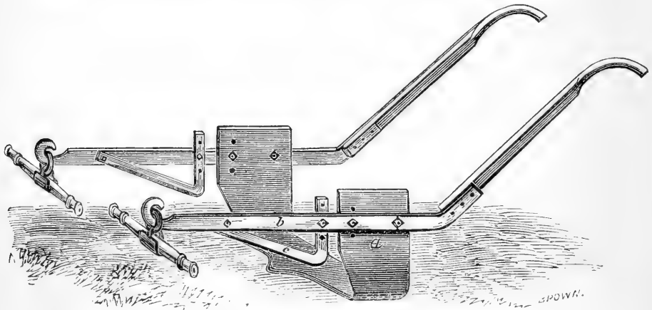
Fig. 23.—HARKNESS' TREE DIGGER.
