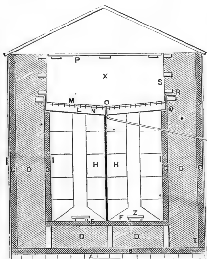
Fig. 27.—NYCE'S FRUIT PRESERVING HOUSE. (CROSS SECTION.)
