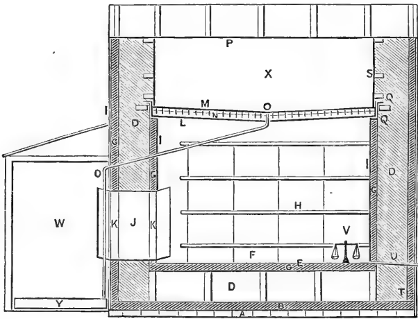
Fig.28.—NYCE'S FRUIT PRESERVING HOUSE. (LONGITUDINAL SECTION.)
