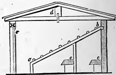
TRANSVERSE SECTION.
