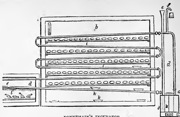
BONNEMAIN'S INCUBATOR.
