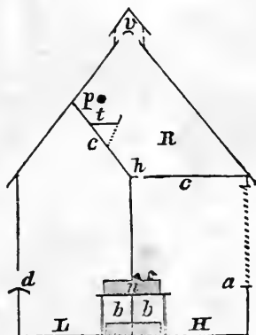
TRANSVERSE SECTION.
