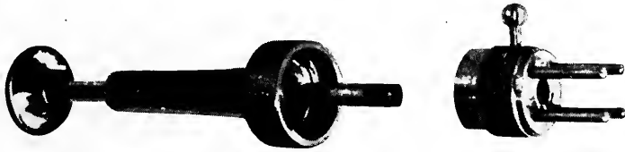
Fig. 94 The Pope false muzzle and bullet starter
