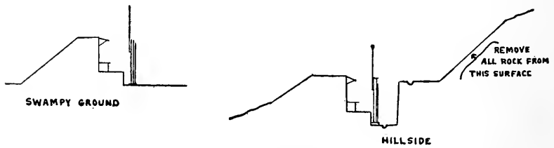
Fig. 171 Showing construction of butts on various sites
