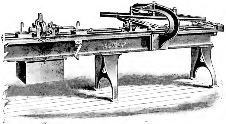
RIFLING MACHINE
