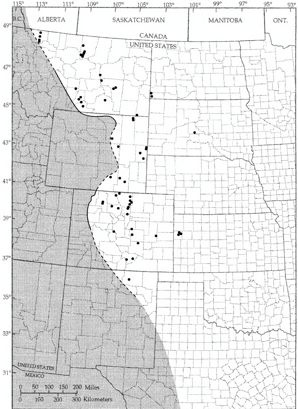
Fig. 5. Western shoreline of the Western Interior Seaway during the time of the Baculites reesei Zone (upper part of the upper Campanian). Dots indicate localities at which B. reesei occurs.
