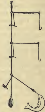
Fig. 16. The Author's Long Boom Straight-Pull Catch Paternoster, for Pier Fishing and Slack Water.
