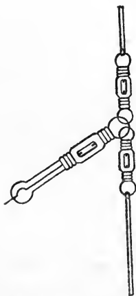
Fig. 15. Jephcott Treble-Swivel.
