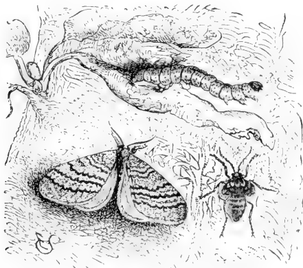
Fig. 35.—Male and Wingless Female of Winter Moth.
