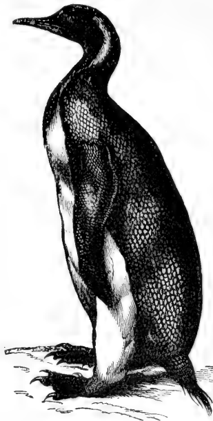
Fig. 7.-- Aptenodytes patagonica (from Brehm).
