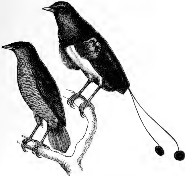
Fig. 32.— Cincinurus regius (male and female).
