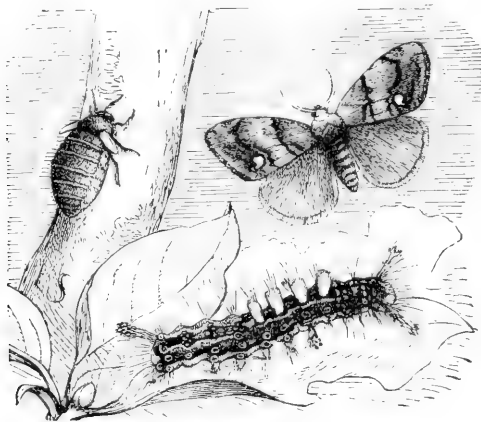
Fig. 17.—Vapourer Moth : male, female, and larva.
