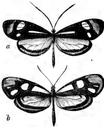
Fig. 24.— a , Leptalis Theonoi , var. Leuconoi (Pieris). b , Ithomia Herdia (the mimicked Heliconius). (After Bates.)
