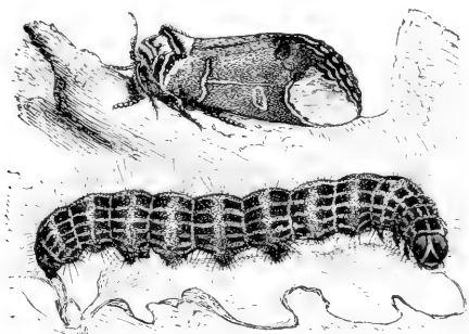
Fig. 15.—Buff-tip Moth and Caterpillar.
