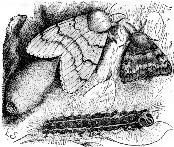
Fig. 36.—Gypsy Moth (male, female, cocoon, and larva).
