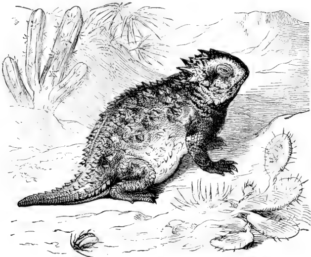
Fig. 13.—The Horned Toad ( Phrynosoma ).
