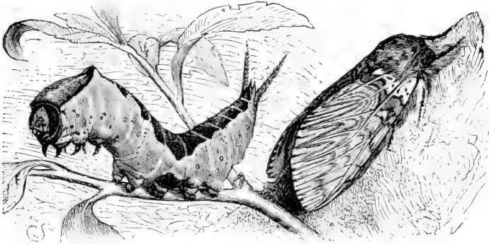
Fig. 11. —Puss Moth and Caterpillar.
