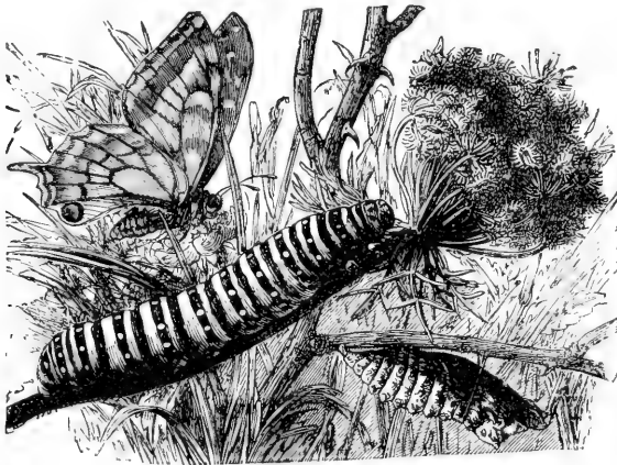
Fig. 18.—Swallowtail Butterfly and Larva.
