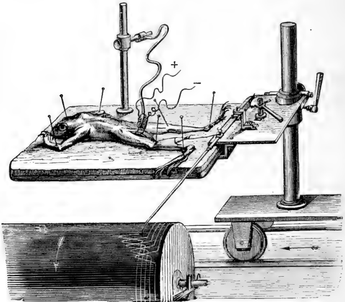
FIG. 3.—Marey's Myograph.
