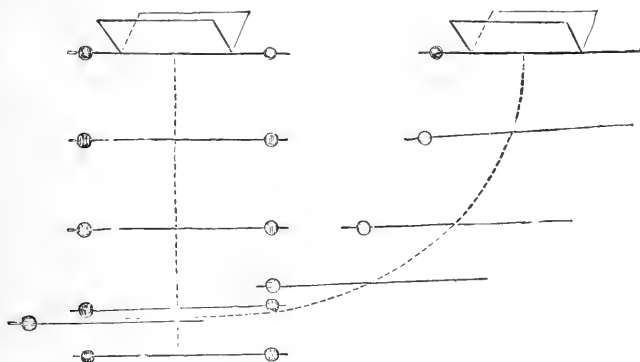
FIG. 90.—R presenting, on the left, a contrivance intended to imitate the hovering of birds; it is placed in equilibrium by two equal weights attached to the extremities of a wire which is fixed in the lower part of the angle formed by the folded paper. This piece of apparatus falls vertically, as shown by the successive positions of the wire when attached to the two weights. On the right is seen the same contrivance connected with one weight only. Its fall is parabolic, as shown by the dotted trajectory.
