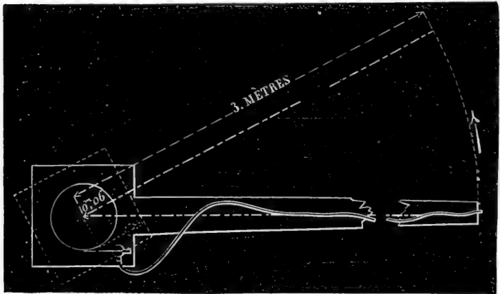
FIG. 24.—Showing two successive positions of the arm of the instrument and the corresponding positions of the tracing points of the levers. The arm of the lever being three metres in length, and the radius of the cylinder being only six centimetres, a similar angular displacement of the person walking, and of the style which writes, will correspond with spaces which will be to each other as 50 to 1.
