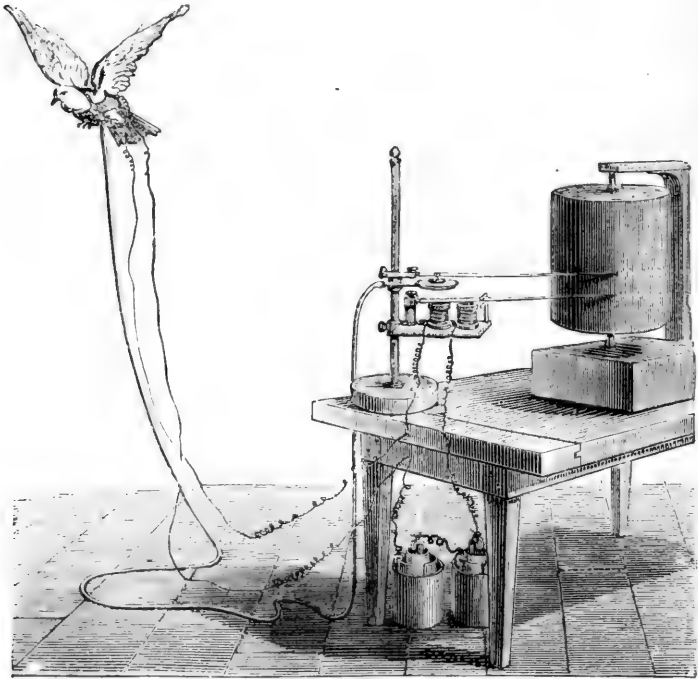
FIG. 91.—Experiment to determine by the electrical and myographical methods, at the same time, the frequency of the movements of the wing and the relative durations of its elevation and depression.
