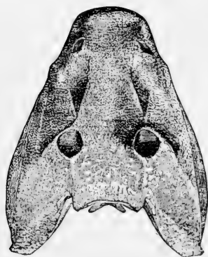
Skull of Eryops , a stegocephalian from the Permian of Texas. Much reduced. (After Cope.)
