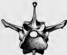
Jaw, vertebra, and single tooth of Hesperornis regalis . The vertebra and jaw are smaller than the originals, and the tooth is twice natural size.
