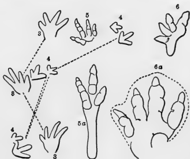
Outlines of dinosaur footprints in the red sandstone of the Connecticut Valley. Very much reduced. (After Hitchcock.)
