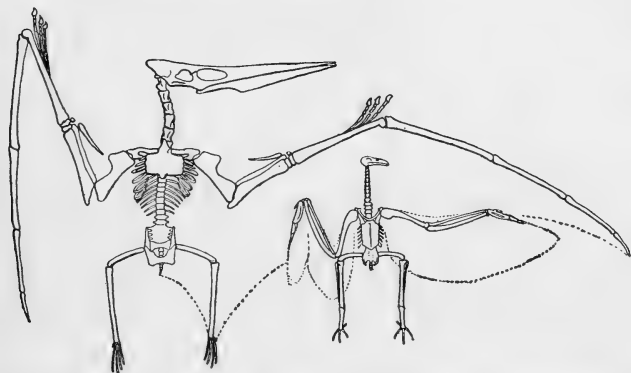
Skeleton of the great pterodactyl Ornithostoma compared with the skeleton of a condor.
