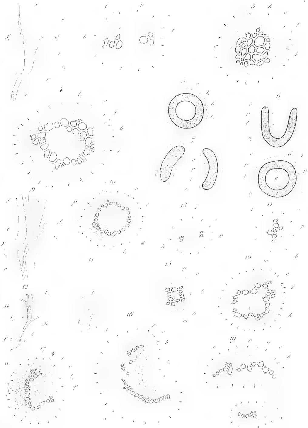
Pteris (1-8), Nephrodium (9-10), Polypodium (11-19).
