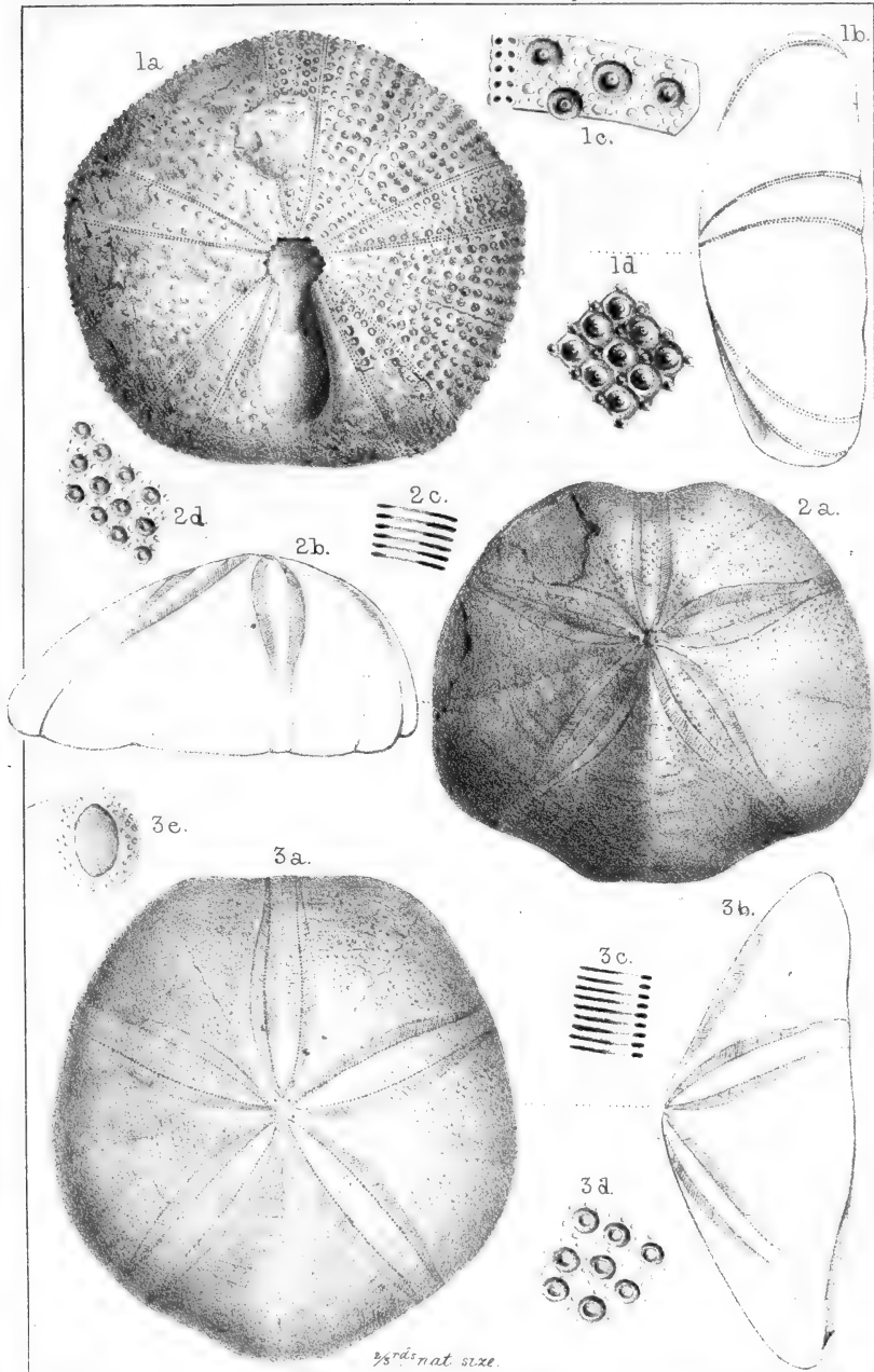
1 a-d Pygaster Morrisii , Wright. 2 a-d Pygurus Blumenbachii , Koch & Dunker. 3 a-e Pygurus pentagonalis , Wright.
