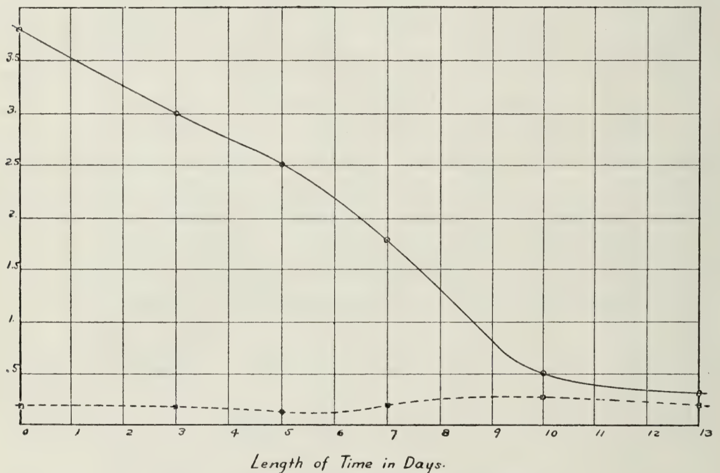
FIG. 17. Ether Extract, grams per 100 seedlings.
