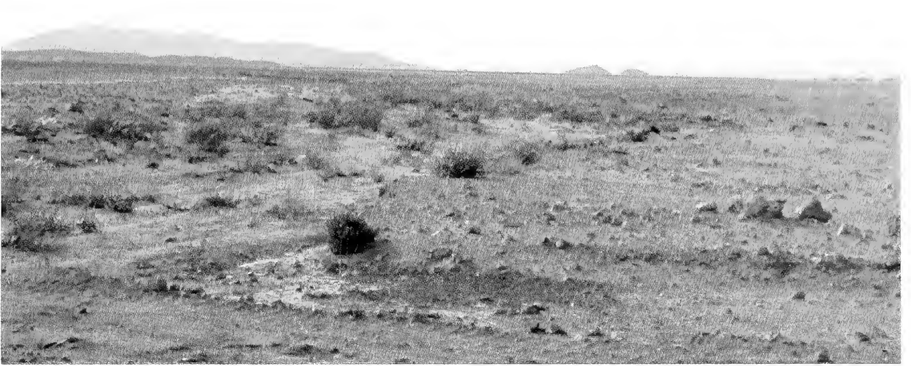
Fig. 15. Drainage channel, east of Walvis Bay, Central Namib Desert.
