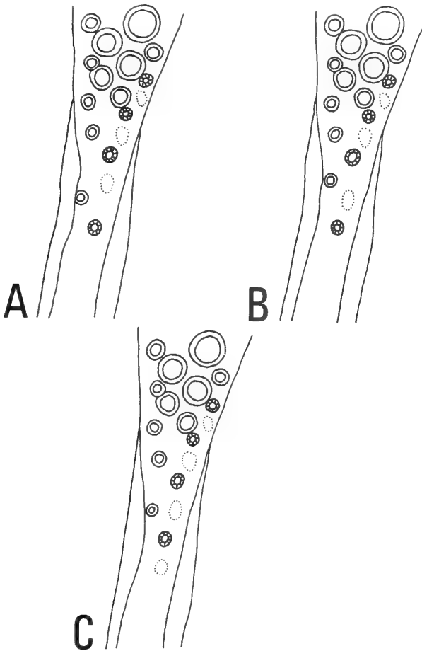
Fig. 4. Three possible variations of the fixing apparatus on the right club of Sthenoteuthis oualaniensis . A. First element of fixing apparatus, a sucker; two suckers proximal to the first knob. B. First element of fixing apparatus, a sucker; one sucker proximal to first knob. C. First element of fixing apparatus, a knob; no suckers proximal to first knob.
