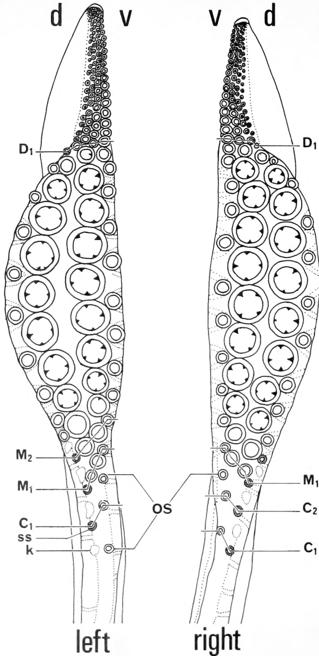
Fig. 1. Semidiagrammatic representation of the tentacular clubs of Sthenoteuthis oualaniensis , mature male, mantle length 126 mm. Galathea sta. 420, 10°24'N 126°40'E. C 1 , C 2 —first and second rows of carpus, d—dorsal, D 1 —first row of dactylus, k—knob of fixing apparatus, M 1 , M 2 —first and second rows of manus, OS—odd (unpaired) suckers of carpus, ss—smooth ringed suckers of fixing apparatus, v—ventral.
