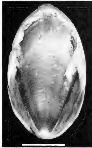
Fig. 11. Sepia pulchra sp. nov. Ventral view of shell of holotype, SAM-S1036, ♂ III 17. Scale = 5 mm.
