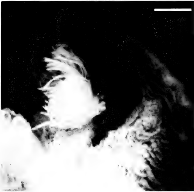
Fig. 13. Sepia pulchra sp. nov. Position of spermatophore bundle on modified portion of hectocotylized left ventral arm; SAM-S1031, ♂ III 17. Scale = 2 mm.
