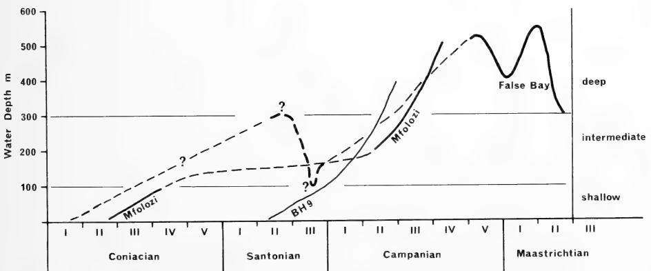
Fig. 43. Water-depth fluctuations during the Upper Cretaceous transgression at three Zululand localities. Based on the CCBC plot (Fig. 39) and Dingle (1980, 1981).
