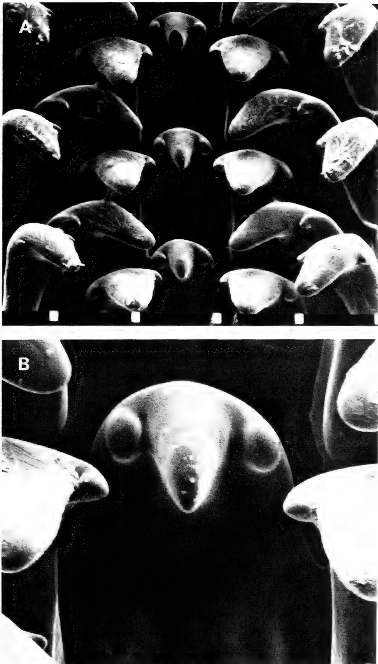
Fig. 6. Cypraea fuscorubra Shaw, 1909. Scanning electron micrographs of teeth. A. Entire width of radula. B. Central region.
