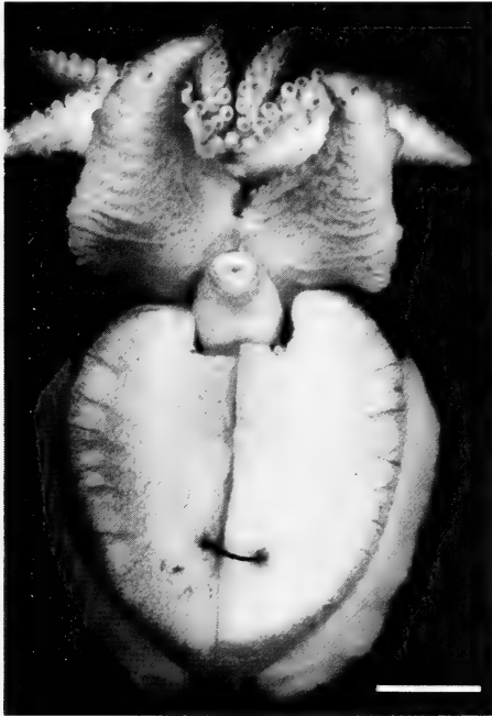
Fig. 2. Sepia pulchra sp. nov. Ventral view of holotype, SAM-S1036, ♂ III 17. Scale = 5 mm.
