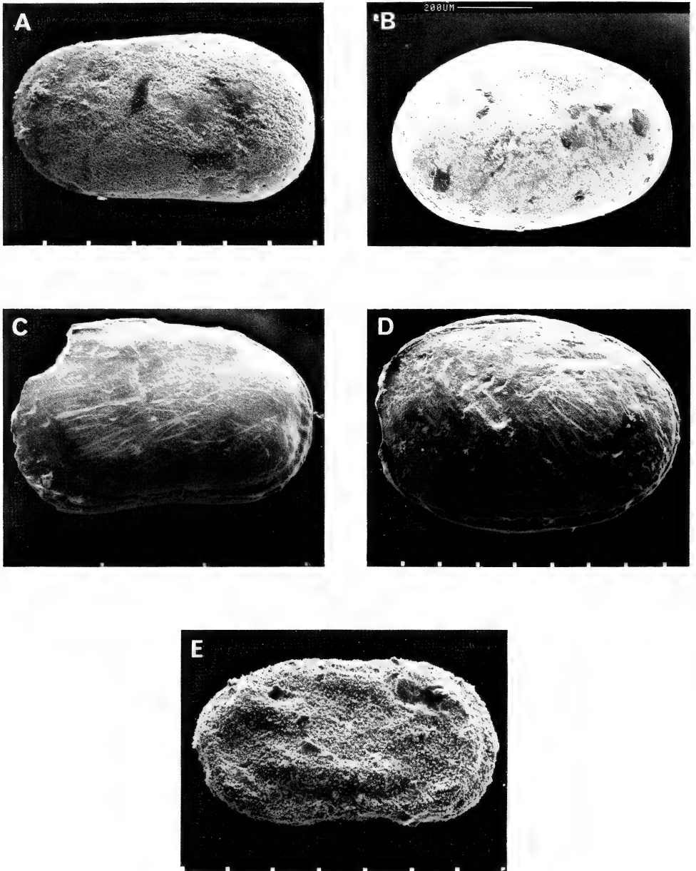
Fig. 5. A. Cytherella sp. 1929, SAM-PC6485, LV, locality 15-5, Mtubatuba, Coniacian IV. B. Cytherella sp. 2351, SAM-PC6486, RV, locality 74-9, False Bay, Santonian III. C. Cytherella sp. 2325, SAM-PC6487, LV, J(c)-1 borehole, 2 115 m, Coniacian. D. Cytherella sp. 2317, SAM-PC6488, LV, J(c)-1 borehole, 2 042 m, Santonian. E. Cytherelloidea mtubaensis sp. nov., SAM-PC6489, holotype, RV, locality 15-1, Mtubatuba, Coniacian IV, SEM 1954. Scale bars: A, D-E = 100 \mu , B = 200 \mu , C = 300 \mu .
