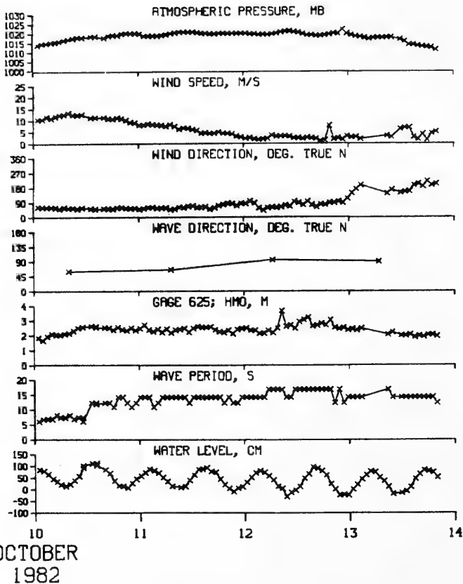
Figure 51. Storm data for 10-13 October 1982
