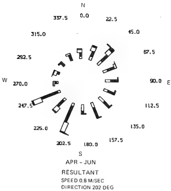
Figure 8. Annual and seasonal wind roses for 1980 through 1982
