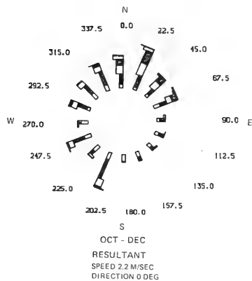
Figure 8. Annual and seasonal wind roses for 1980 through 1982
