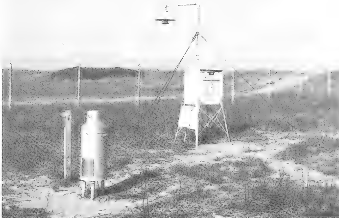
Figure 3. Louvered instrument shelter (background) and rain gages (foreground)
