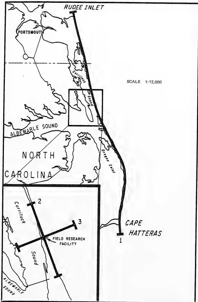
Figure 5. Quarterly aerial photography flight lines, 1981
