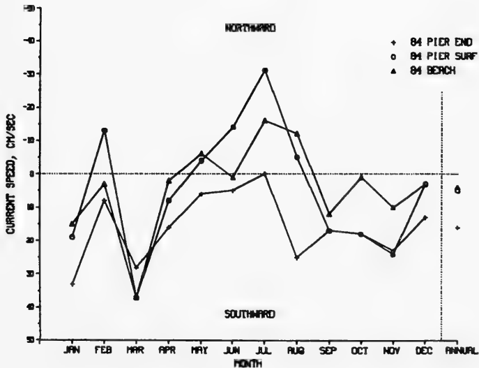
Figure 26. Monthly mean currents, 1984
