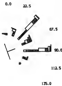
JAN - MAR RESULTANT HEIGHT 1.0 m DIRECTION 63 DEG
