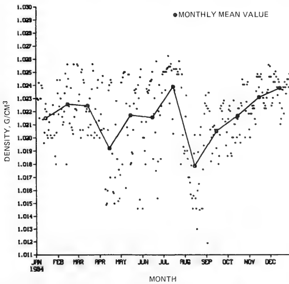
Figure 40. Daily sea surface water density, 1984
