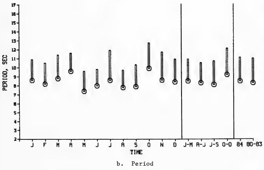
Figure B21. 1984 mean, standard deviation, and extreme H_m and T_p for gage 620
