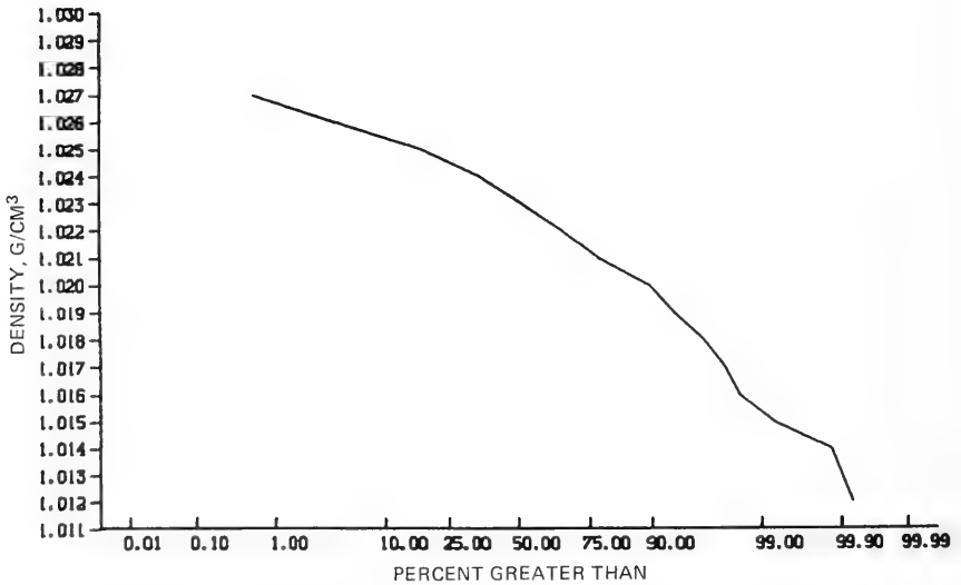
Figure 42. Distribution of surface water density, 1981-1984
