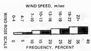
Figure 8. Seasonal wind roses, 1984
