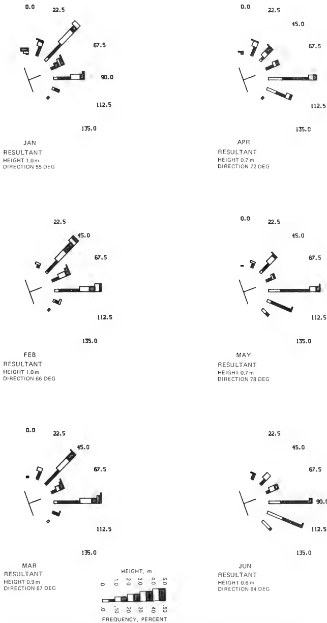
Figure B19. 1980 through 1984 monthly visual wave observation roses (Continued)
