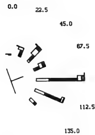
Figure 24. Annual and seasonal wave roses, 1980-1984
