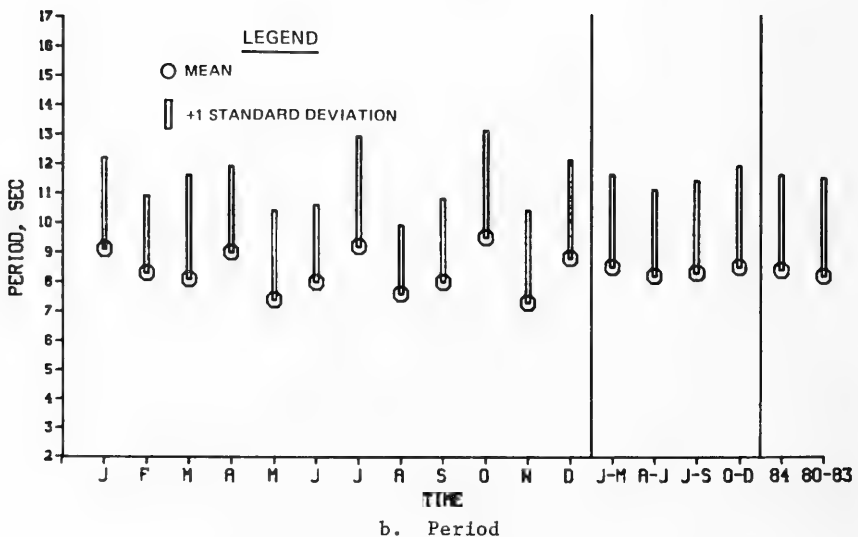
Figure B34. 1984 mean, standard deviation, and extreme H_{m0} and T_p for gage 615
