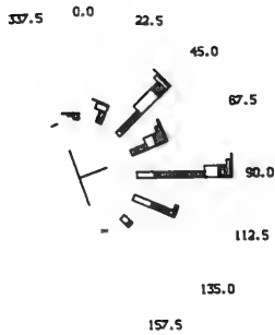
ANNUAL RESULTANT HEIGHT 0.8 m DIRECTION 68 DEG
