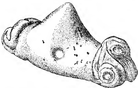
FIG. 36.—Mammiform stone, with the head of a sea-bird. \frac{1}{2} .
