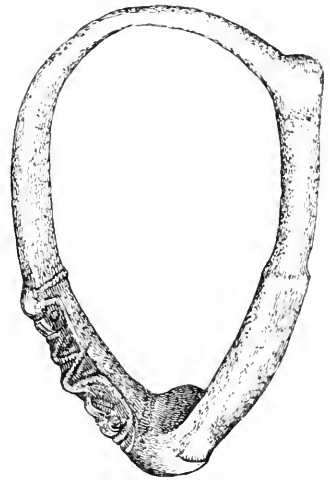
FIG. 59.—A left-shouldered slender collar, showing the shoulder-swelling, the boss, and the panel-border. \frac{1}{2} .
