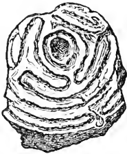
FIG. 9.—Bottom of a vase with the pattern traced in it. \frac{1}{2} .
