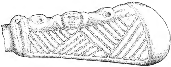
FIG. 57.—Right panel of a left-shouldered slender collar. \frac{1}{2} .
