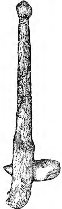
FIG. 12.—Celt of jadeite in a handle of wood, Turk's Island. \frac{1}{2} .
