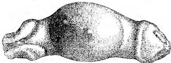
FIG. 37.—Mammiform stone, upper view, greatly warped. \frac{1}{2} .
