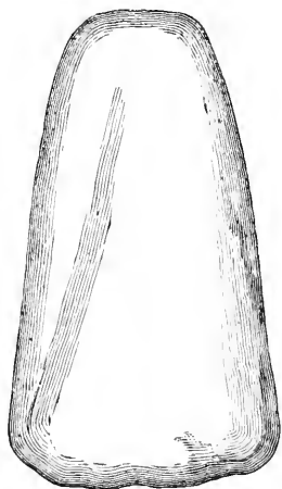
FIG. 15.—Flat-sided truncated celt †
