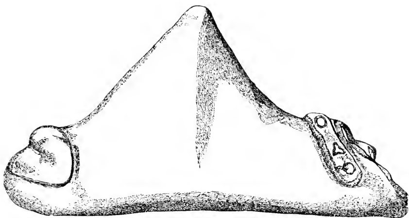
FIG. 35.—Mammiform stone, with human face. About \frac{1}{2} .
