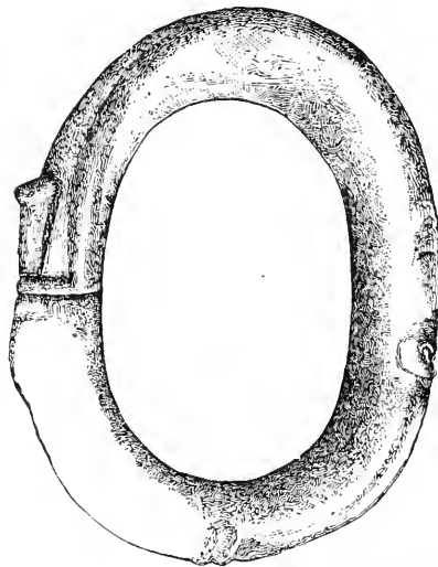
FIG. 51.—Right-shouldered massive collar. \frac{1}{6} .
