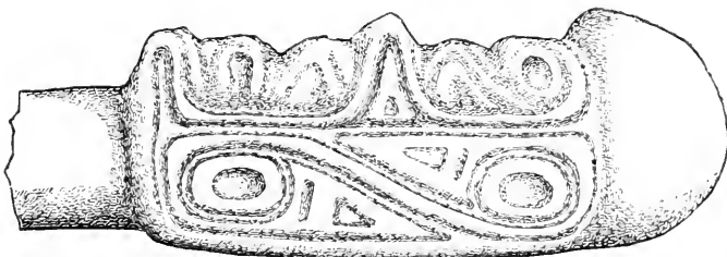
FIG. 60.—Right panel and scrolled border of a left-shouldered slender collar. \frac{1}{2} .
