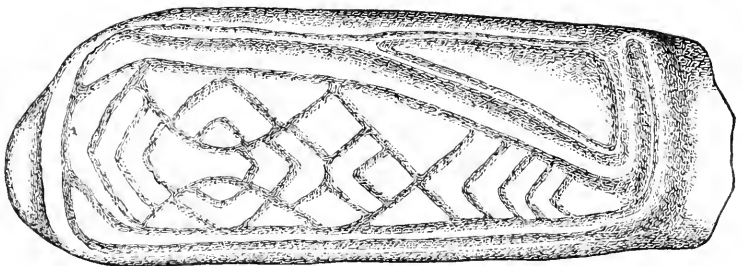
FIG. 52.—Gourd-shaped panel of a massive collar, with its ornament. \frac{1}{4} .
