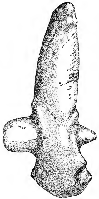
FIG. 11.—Celt and handle of polished jadeite. \frac{1}{2} .
