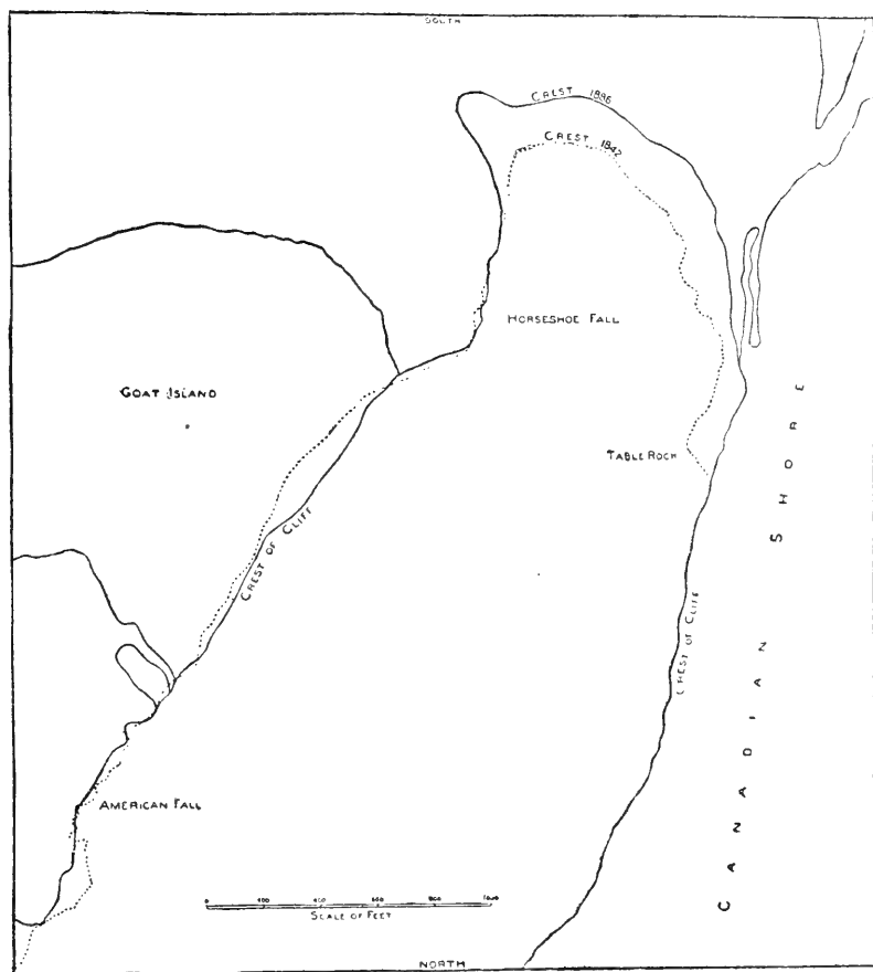
PLATE VII.—CHART OF THE CLIFF LINE AT THE HEAD OF THE NIAGARA GORGE, COMPILED TO SHOW THE RECESSON FROM 1842 TO 1886.
