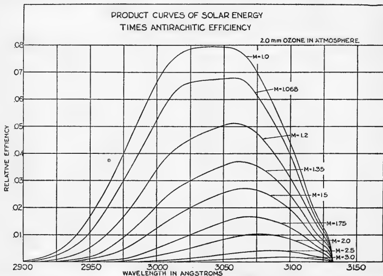
FIGURE 9.—Product curves of solar spectral energy by antirachitic efficiency. (2.0 mm. ozone in zenith atmosphere.)
