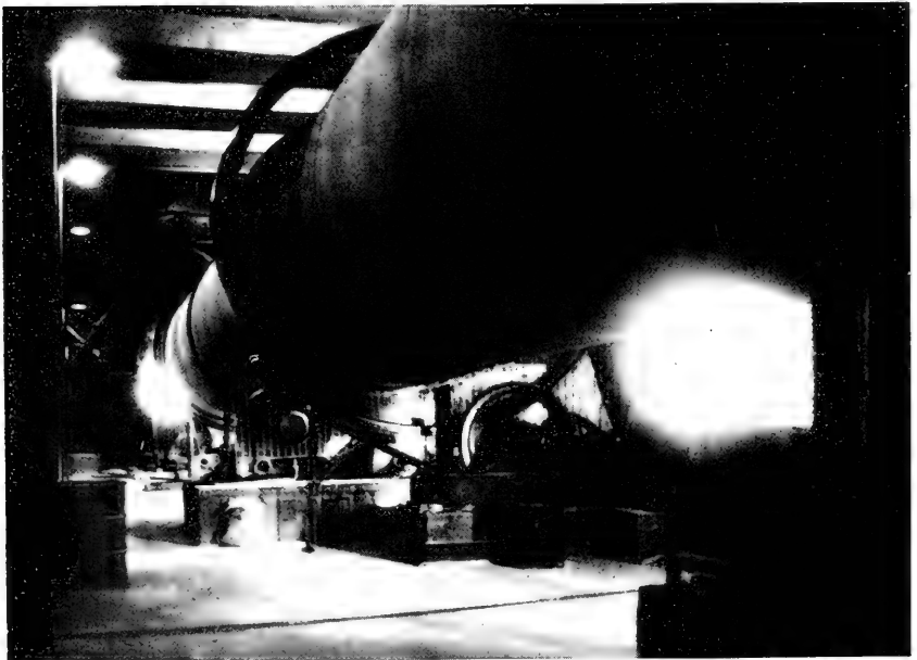
2. THE ROTARY KILNS, WHICH ARE 160 FEET LONG AND 10 FEET IN DIAMETER, EACH BURNS APPROXIMATELY 300 TONS OF MAGNESIA PER WEEK.
