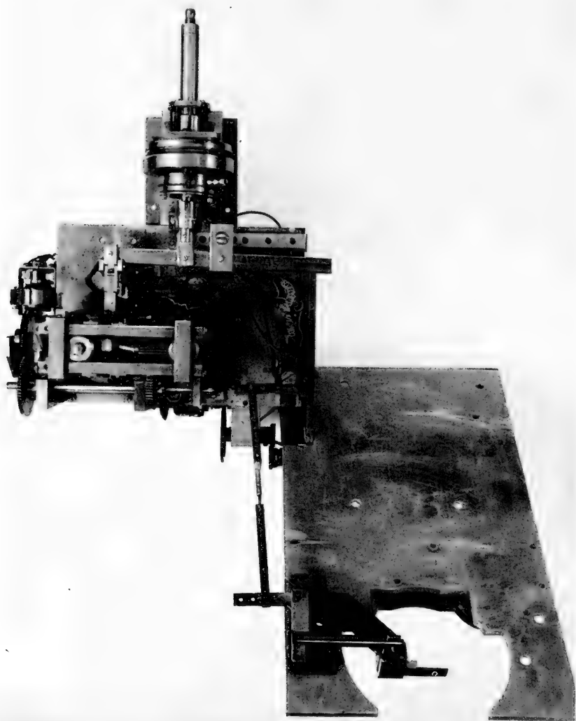
DIAPHRAGM PUMP INJECTOR OF VARIABLE THROW GOVERNED BY DIFFERENTIAL HEAT EXPANSION BETWEEN BOILER AND INVAR TAPE. Rollers which support the mirror seen behind the aluminum plate.
