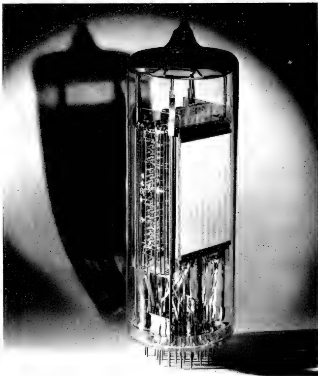
1. THE SB-256 TUBE, AN EFFICIENT ELECTRONIC MEMORY
