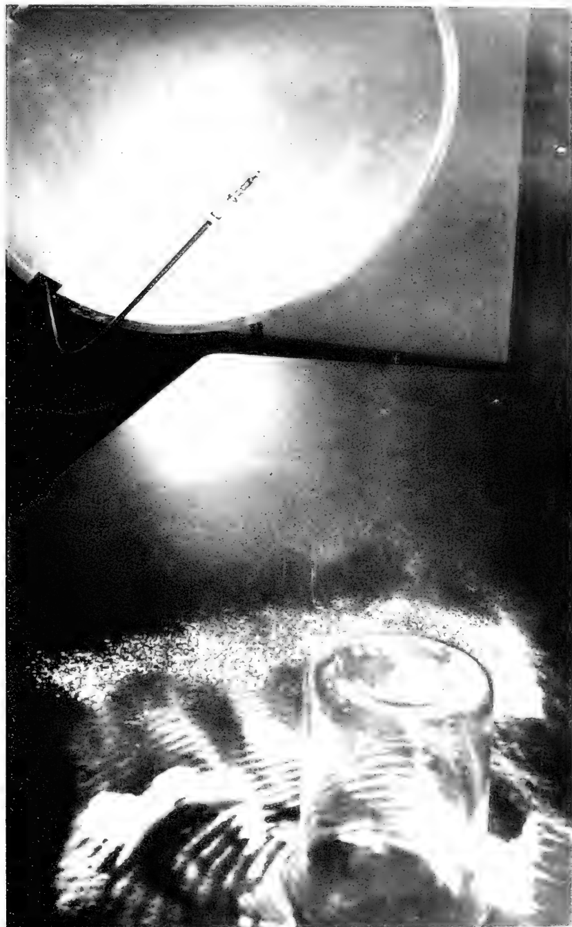
Ultrasonic waves, coming from the tiny whistle, are reflected onto the table by the concave metal disk. The ripples, formed in the water, show the standing waves formed by reflections from the table top and water. C. General Electric Co.
