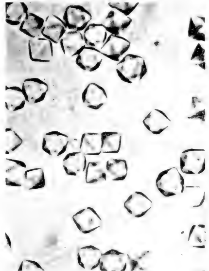
4. Photomicrograph of amylase crystals, \times 800 . This enzyme was the first one to be obtained as crystals. (From Enzymes , by Sumner and Somers.)
