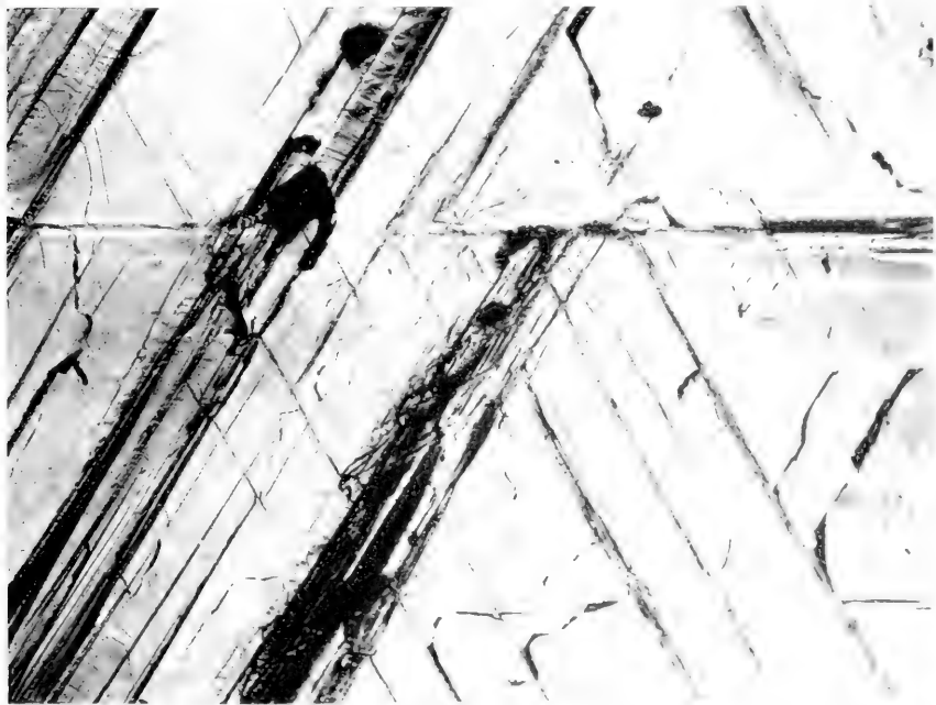
2. Fractograph or photomicrograph of an unpolished surface of metallic bismuth, showing geometric markings and fracture. Magnified 35 times.
