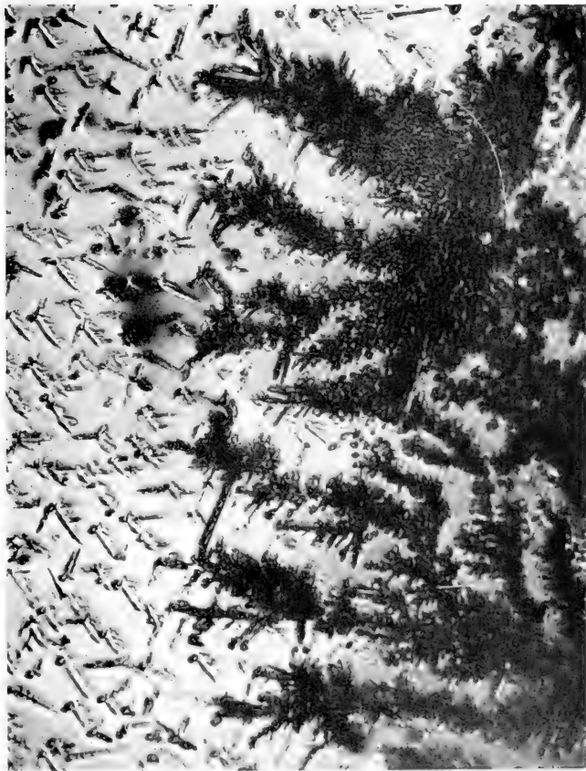
FIG. 1. Fractograph of metal, showing the external surface of a grain (grain boundaries). Oxide was deposited on growths which strongly affect the forgeability. The growths are in the form of thin plates which are carbides, the essential factor for forgeability. The growths are in the form of thin plates which are carbides, the essential factor for forgeability. The growths are in the form of thin plates which are carbides, the essential factor for forgeability. The oxide was removed by the vacuum treatment. The oxide was removed by the vacuum treatment. The oxide was removed by the vacuum treatment. Magnified 385 times.
