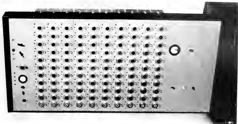
2. AN ELECTRONIC ANALOGUE COMPUTER THE SIM III — TANEUS EQUATION SOLVER
