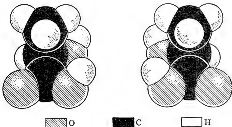
FIGURE 1.—Models of the two forms of lactic acid, \text{CH}_3\text{CH}(\text{OH})\text{COOH} , which are mirror images. These models give the best representation that is possible of the actual shape of molecules. (From Organic Chemistry , by L. F. and M. Fieser.)
