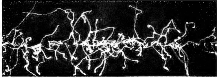
2. Traces of electrons photoelectrically ejected from molecules of air by X-rays. From G. Amaldi, Misleri della Materia , Milan, 1950.
