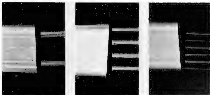
2. Transmission of a wide ultrasonic beam through aluminum wedges of increasing taper. Transmission occurs only where the wedge thickness is such as to give internal resonance. Courtesy Bell Laboratories Record .
