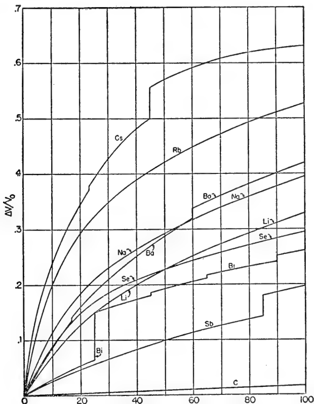
FIGURE 4.—The change of relative volume of a number of substances shown as a function of pressure up to 100,000 kg./cm. 2 (metric atmospheres).
