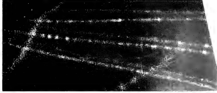
3. Cloud-chamber photograph of a particle electron shower. From Montgomery, Cosmic Ray Physics , Princeton, 1949. Courtesy Dr. Wayne E. Hazen.
