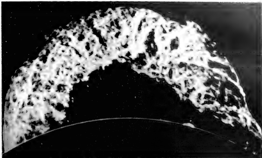
1. Large eruptive prominence of June 4, 1946, photographed in hydrogen light, 6563 Å. The prominence is shown rising in an enormous arch above the edge of the artificially eclipsed sun. The immense cloud of hydrogen rose to a height of hundreds of thousands of miles in less than 2 hours.
