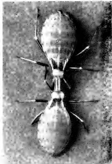
FIGURE 4.— Rhodnius larva in 4th stage decapitated 1 week after feeding and connected by means of a capillary tube with another 4th-stage larva decapitated 24 hours after feeding. The molting hormone from the first insect causes the second to molt. \times 3 .
