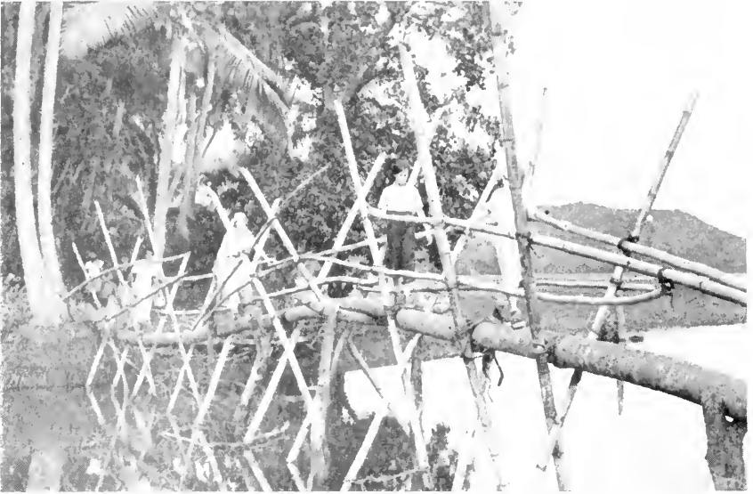
1. A footbridge of palm trunks and bamboo stems crosses a tidal creek on Ngau. The Fijians are adept builders with local materials, and such a temporary fiber-lashed structure is made in a matter of minutes.
