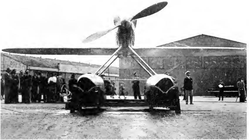
1. The world's-record supermarine seaplane (1929). Necessary propeller clearance and high center of gravity made this a heavy, awkward plane, with greatly added head resistance.
