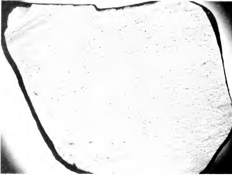
2. Libyan Desert glass, showing internal structure of a thin polished section by means of transmitted light.
