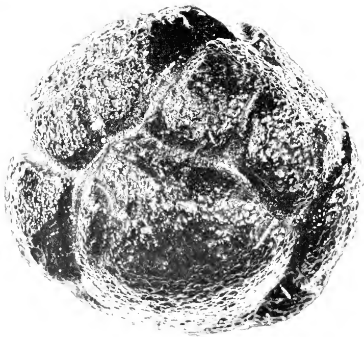
1. Tektite from Paracale Bay, Philippines, illustrating surface features often found on tektites recovered within that area.
