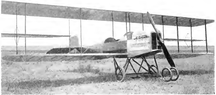
1. America's first highly successful tractor type, the Glenn Martin training plane of 1913. Note useless skids and nose wheels on the landing gear; also ailerons between the wings.
