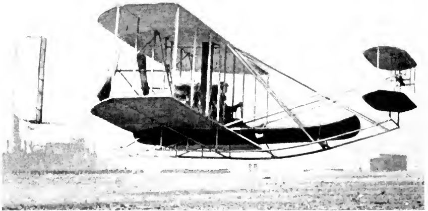
1. The Wright Model A of 1909, with canoe attached for Hudson-Fulton flights over New York harbor. Skid landing gear, no wheels, no rear horizontal tail.
