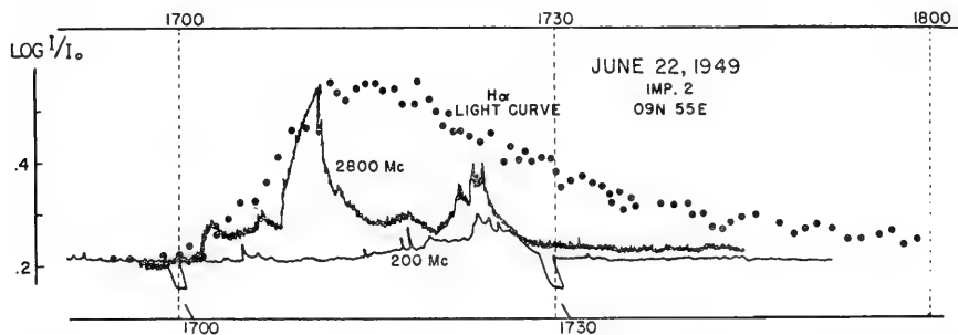
FIGURE 3.—Comparison of H\alpha flare light curve (McMath-Hulbert Observatory) and concomitant 2800 Mc/s and 200 Mc/s solar radiation. The two radio-frequency records were recorded at N.R.C. (Ottawa) and Cornell University, respectively.
