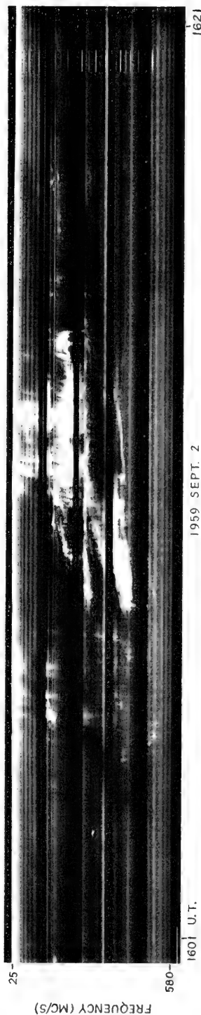
Sweep frequency records of solar radio bursts on May 10, 1959, and September 2, 1959, taken at the Harvard Radio Astronomy Station, Fort Davis, Tex. These bursts were caused by disturbances moving outward through the solar atmosphere at approximately 1,000 km. per second. Both the bursts were followed approximately 30 hours later by terrestrial magnetic storms.
