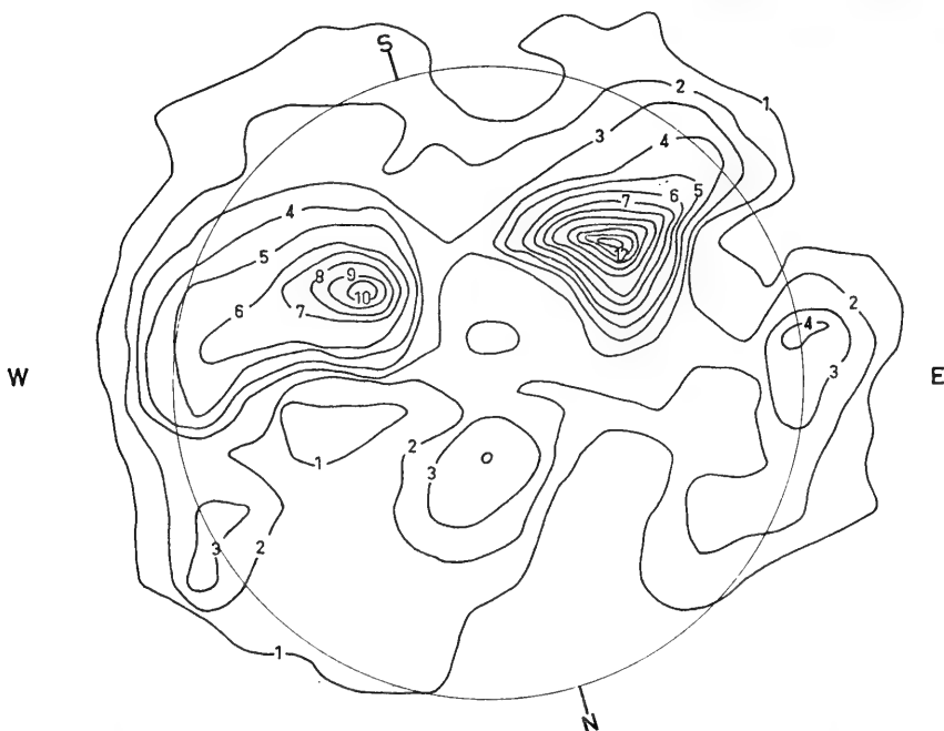
FIGURE 1.—Radioheliogram of the sun at 21 cm. The contour brightness unit is 0.93 \times 10^8 °K. (Diagram courtesy of Dr. W. N. Christiansen, CSIRO Division of Radio-physics, Sydney, Australia.)
