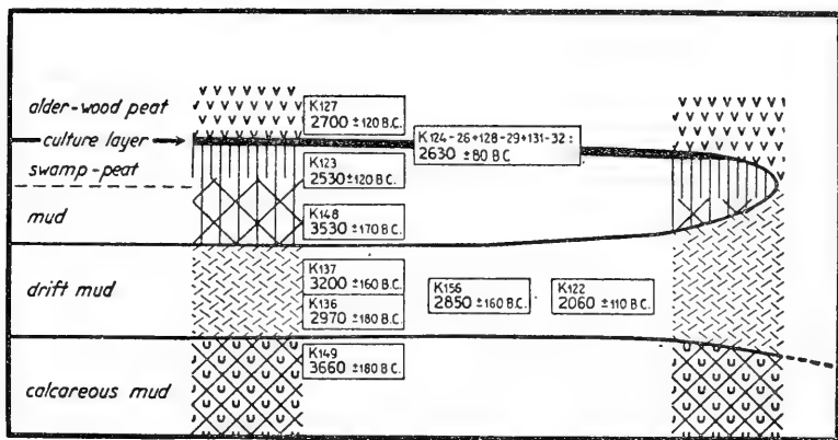
FIGURE 17.—Schematic section through the dwelling place on the floating peat island. K-123, etc., are the numbers of the carbon-14 samples. All dates given are B.C. According to a correction from the radiocarbon laboratory all dates should be 200 years older.
