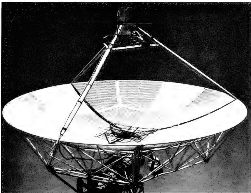
2. The 28-foot antenna and 4-octave primary feed system used for solar radio observations at the Harvard Radio Astronomy Station, Fort Davis, Tex.
