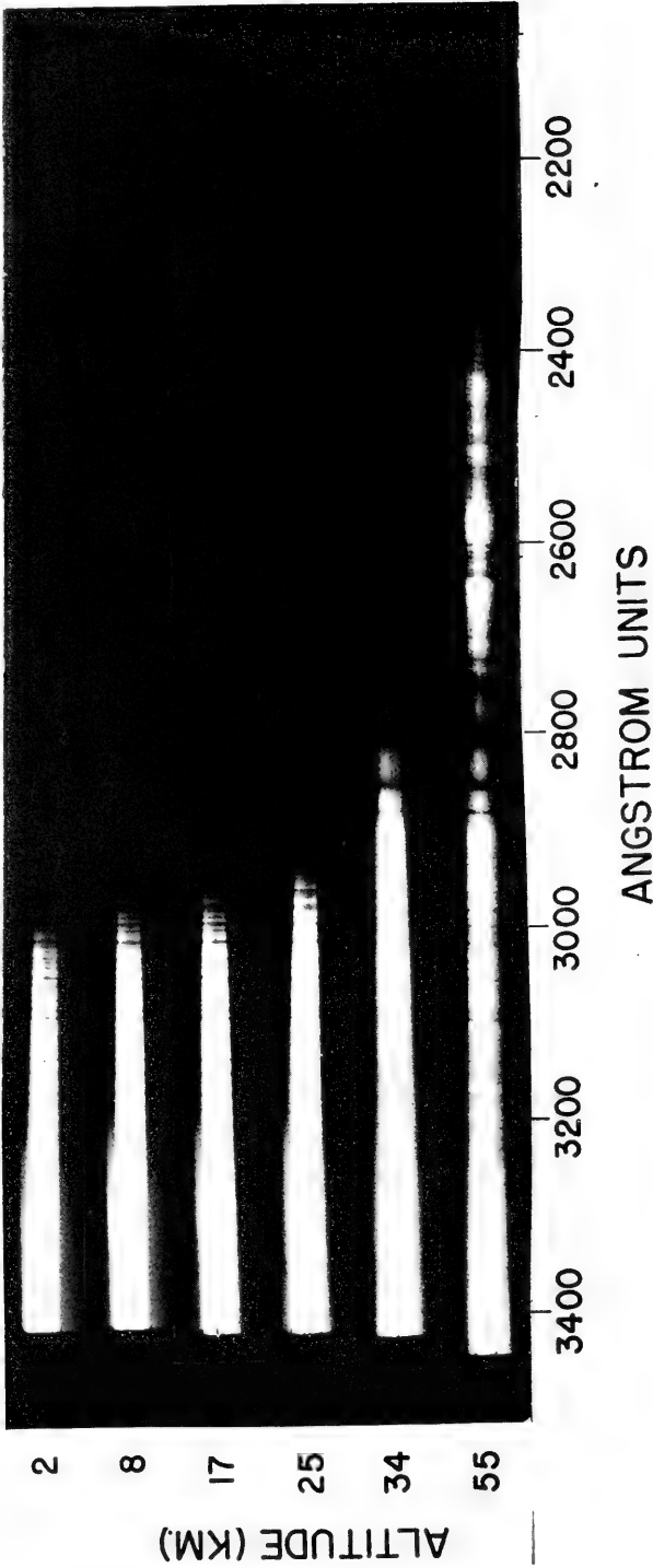
The first solar spectra recorded above the ozone layer. Photographed from a V-2 rocket on October 10, 1946, by the U.S. Naval Research Laboratory.
