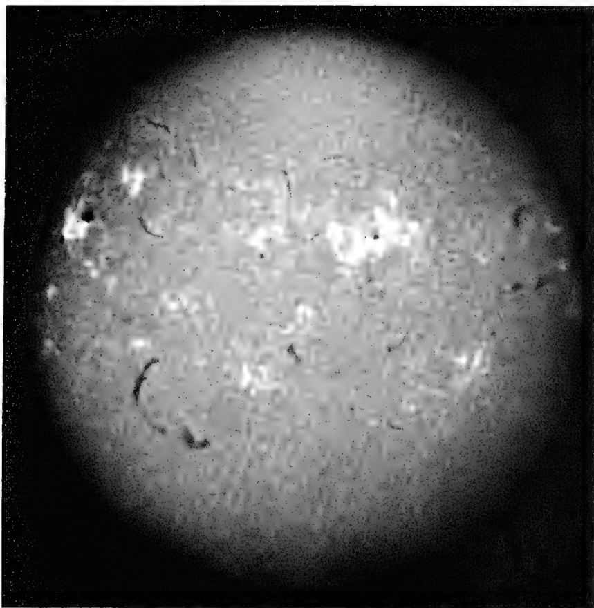
H \alpha filterheliogram showing filaments, plages, and three flares, 1959, June 18 d 11 h 44 m U. T. Flare, importance 3, N17 W13, near maximum; importance 2, N06 E60, past maximum; importance 1, N19 E47, near maximum. (North is at the top, east is at the left.) McMath-Hulbert Observatory of the University of Michigan.
