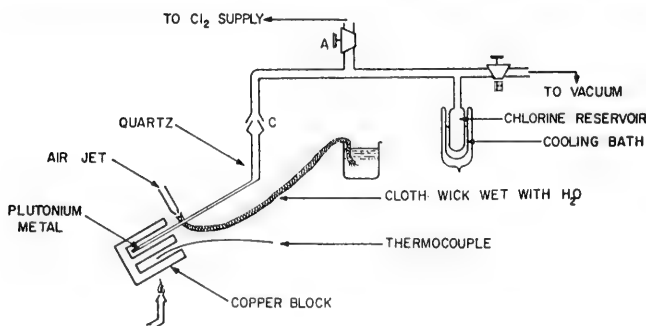
FIGURE 3.—Apparatus used in the first preparation of \text{PuCl}_3 (February 1944). The compound was prepared by treating a 50\text{-}\mu\text{g} piece of plutonium metal with chlorine gas. After placing the plutonium in the capillary tube, the system was evacuated. Chlorine gas was added, and a small amount condensed in a reservoir as shown. The system was closed and remained filled with chlorine at a pressure of about 60 mm. Hg. The copper block was heated to 45^\circ\text{C} ., and the reaction product was formed in the top of the capillary tube. The section of the capillary containing the product was sealed off and the compound formed was identified by X-ray diffraction.
