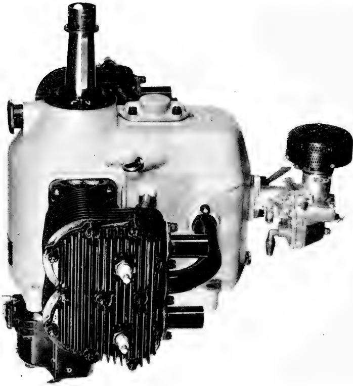
1. Continental A-40, 4-cyl. horizontal opposed, 38 hp., 1931.
