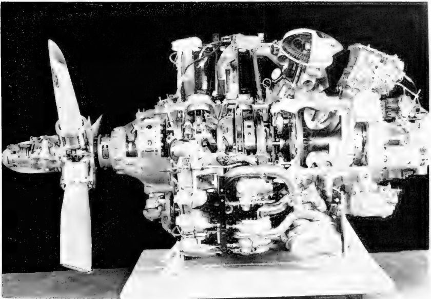
2. Wright turbo-compound, 18-cyl., 2-row air-cooled radial engine, 3350 hp., 1946 (cutaway).
