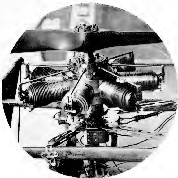
1. Gnome engine, 1910, 7-cylinder rotary, 50 hp., 1910.
