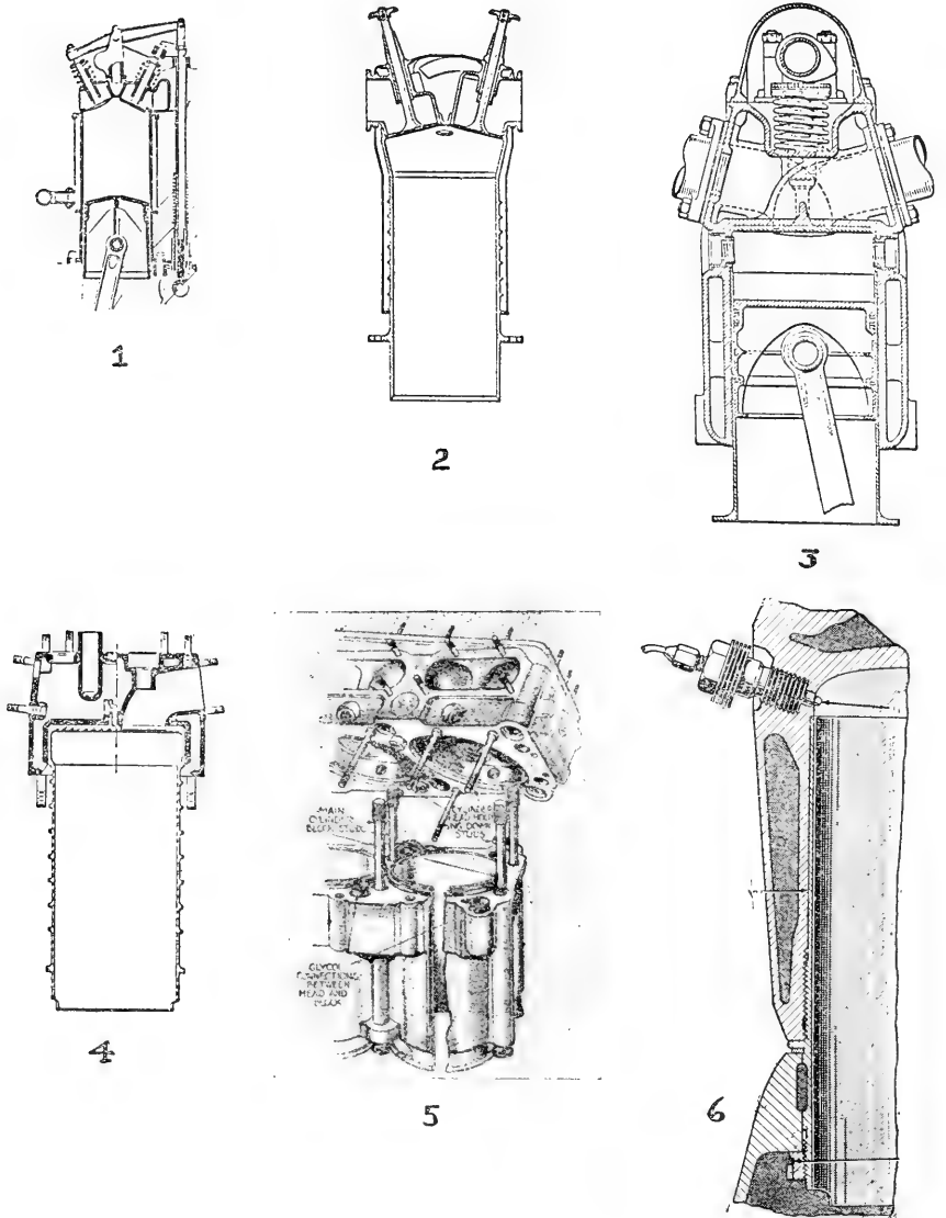
FIGURE 10.—Liquid-cooled cylinder development.
