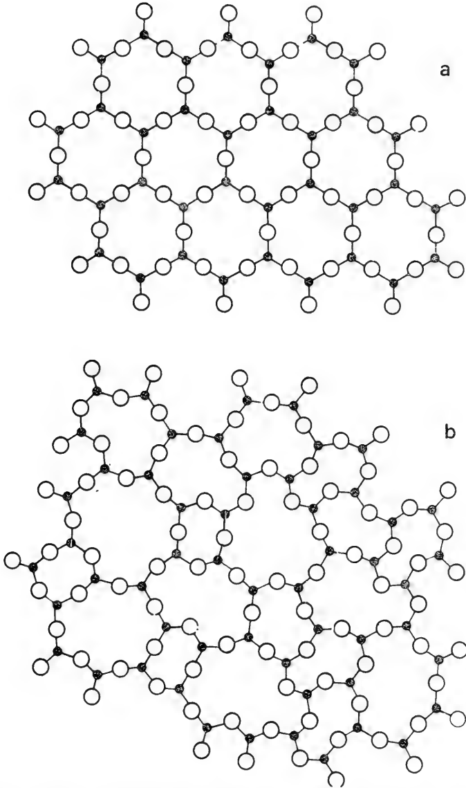
FIGURE 2.—Schematic two-dimensional representation according to Zachariasen of structures of \text{SiO}_2 network former: a , crystal; b , glass.
