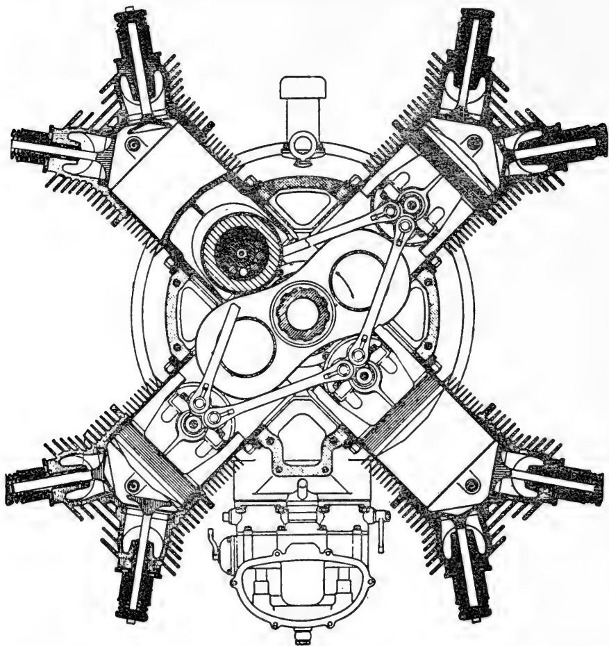
FIGURE 19.—Fairchild-Camenez engine, transverse section. This was the only crankless reciprocating engine to reach the stage of official approval (U.S. Dept. of Commerce Approved type Certificate No. 1, June 1927). Later it was found to be impractical because of severe torque variation.
