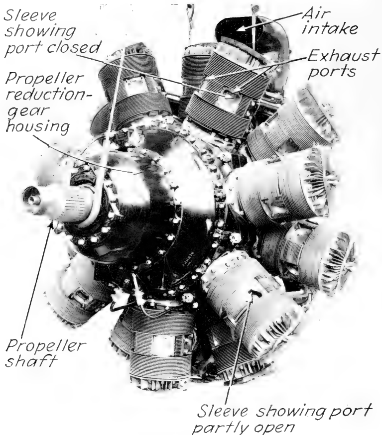
1. Bristol "Hercules" sleeve-valve engine, 14-cyl., radial air-cooled, 1650 hp., 1948. (Courtesy Bristol Aeroplane Co., Ltd.)
