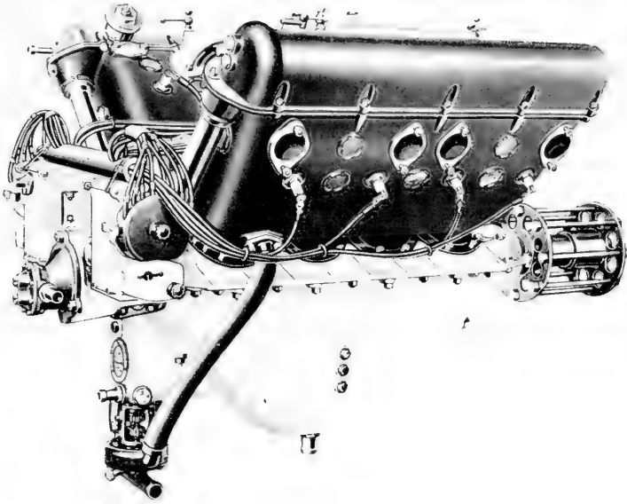
1. Hispano-Suiza engine, V-8, 180 hp., oblique view, magneto end, 1915.
