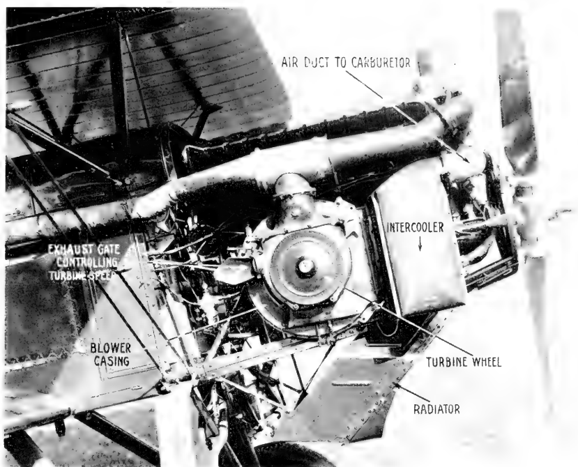
1. Side type turbo-supercharger installation on Curtiss D-12 engine, 460 hp., in Curtiss Falcon airplane, 1931. (Courtesy Materiel Div., U.S. Air Force.)
