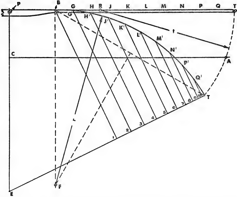
FIGURE 6.—Graphic method of designing a bow. BT , the limb, is divided into ten equal sections. Its tip, in bending, follows the path TT' , a circular arc with center at R and radius r , which is 3/4 BT in length. The length of the arrow is EP ; the line CA represents the string on the braced bow, with CP the "bracing height"; ET' represents the string at full draw. Arc BT' represents the bent limb, with radius r , the center of which is located by the intersection of the line BF which is perpendicular to BT , and the perpendicular bisector of chord BT' . Perpendiculars to ET' are dropped from each of the ten equally spaced points B, G', H', \dots, Q' , along the bent limb. The lengths of the perpendiculars are proportional to the respective widths of the limb at each of the ten locations.
