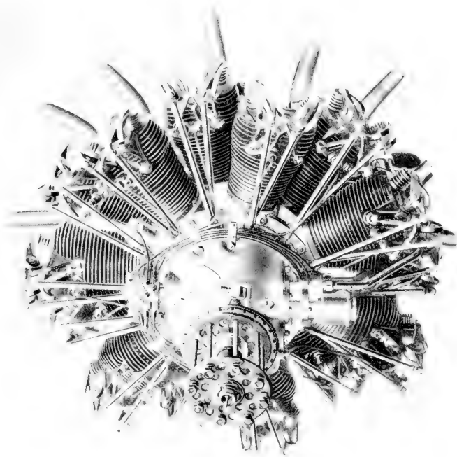
2. Armstrong-Siddeley Jaguar, 1922. First successful British radial engine with aluminum-head cylinders and gear-driven supercharger.
