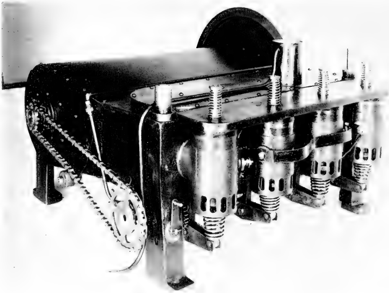
1. Wright brothers' engine from 1903 airplane.
