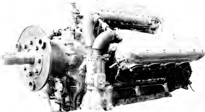
2. Napier "Lion" 12-cyl. "W"-type liquid-cooled engine. The only example of this form ever widely used. Normal rating, 450 hp. A racing version of 800 hp. powered the winner of the Schneider Trophy for seaplane speed in 1927, the Supermarine S-5 which flew at 281.65 m.p.h.
