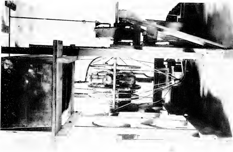
1. Langley-Manly-Balzer engine, 1903 in test stand.
