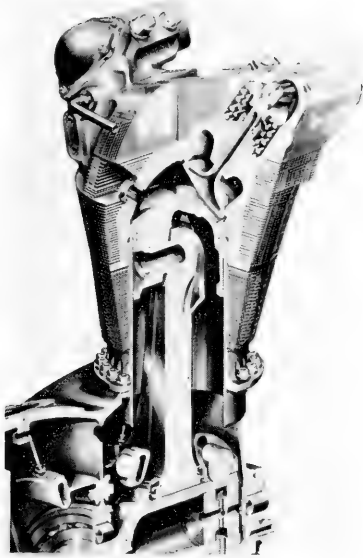
1. Forged cylinder for Wright 3350 engine, 1948. Forged and machined head, steel barrel with aluminum fins rolled in, sodium-cooled valves Stellite-faced, 100-plus square inches of fin area per square inch of piston area. (Courtesy Wright Aeronautical Corp.)
