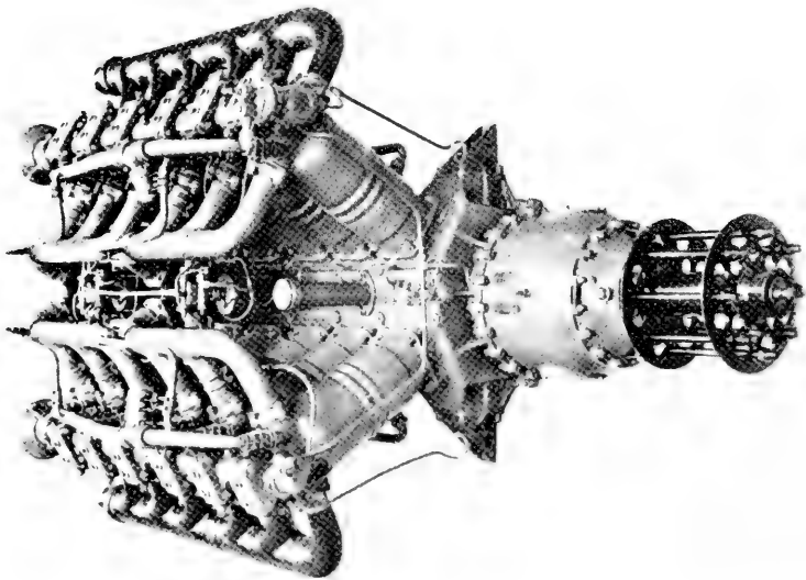
1. Rolls-Royce "Eagle" engine, 12-cylinder Vee, 360 hp., England, World War I.
