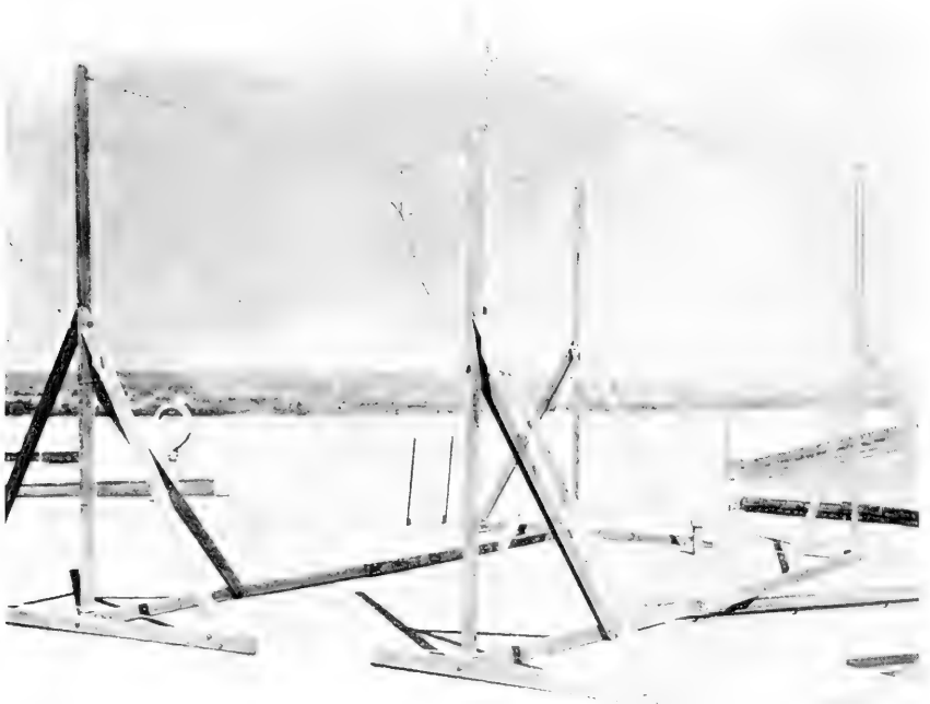
2. Original 28-Mc radar receiving antenna; \lambda/2 dipole with \lambda/2 reflector. April 1936.
