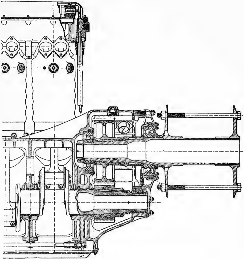
FIGURE 17.—Reduction gears of Renault Type 12 Kh engine.
