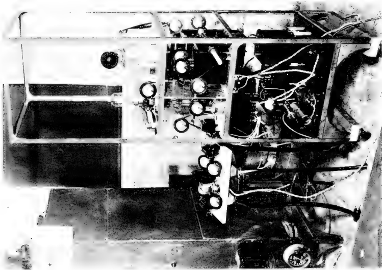
1. Original 28-Mc radar transmitter with synchronizing keyer. 17,000 v on exposed wires and condensers on top shelf. April 1936.
