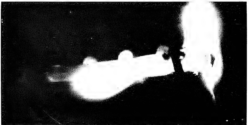
2. Night view of a turbo-supercharger in operation, the same installation as in fig. 1 above. The exhaust manifolds and the nozzle box are white hot from the high temperature of 1500° F., and the turbine is surrounded by hot gases while operating at over 20,000 r.p.m.
