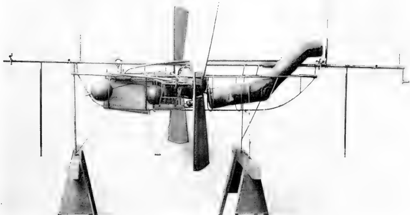
1. Langley steam engine used in Aerodrome No. 5, 1896.
