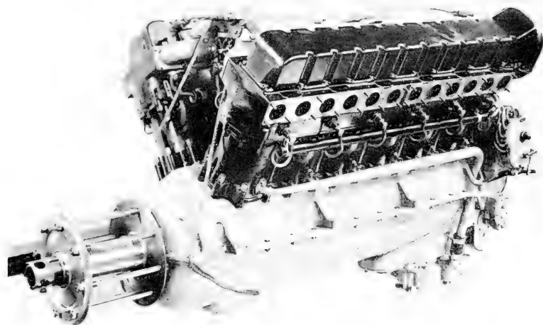
1. Curtiss D-12 engine, first to fly more than 200 m.p.h., Detroit, 1922.
