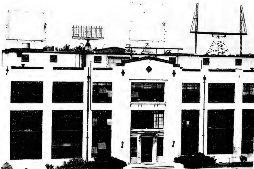
2. Penthouse roof, Bldg. 12, showing (right to left) pre-XAF, XAF, 400-Mc, and CXAM antennas. Pre-XAF is hand driven; all others are motor driven with remote control. Summer 1940.
