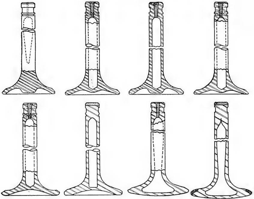
FIGURE 14.—Evolution of Wright Cyclone engine valves. From Journal of S.A.E. , Colwell, 1940.
