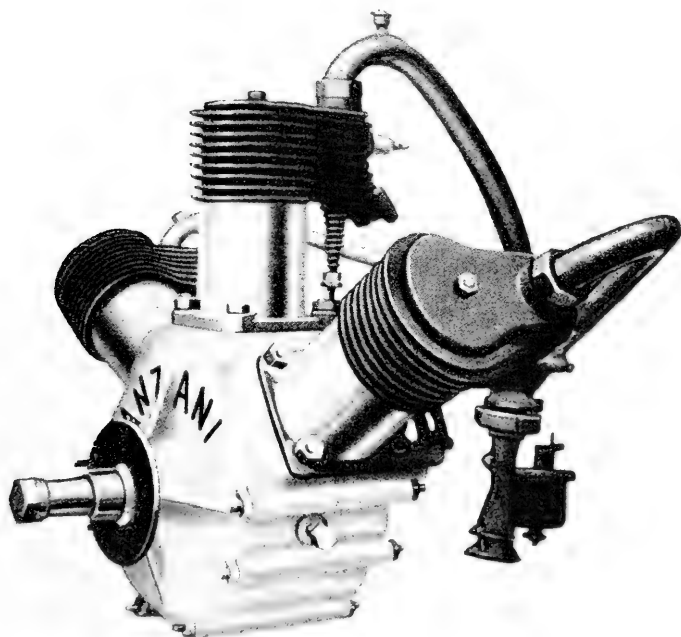
2. Anzani 3-cylinder fan-type engine, 22 hp., 1909.
