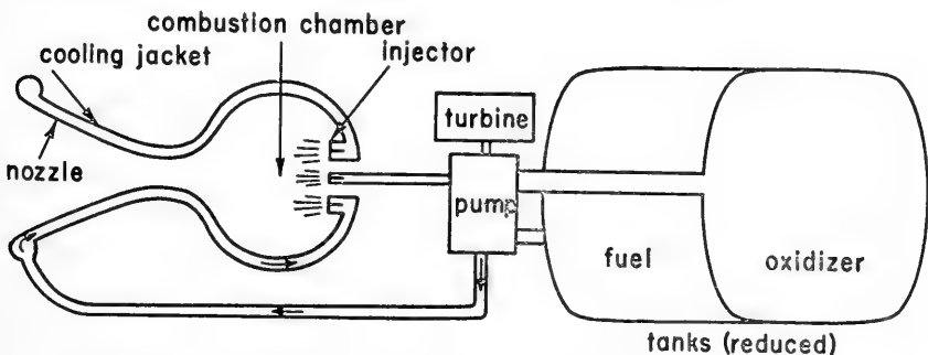
FIGURE 2.—Simplified schematic of a typical liquid propellant rocket.
