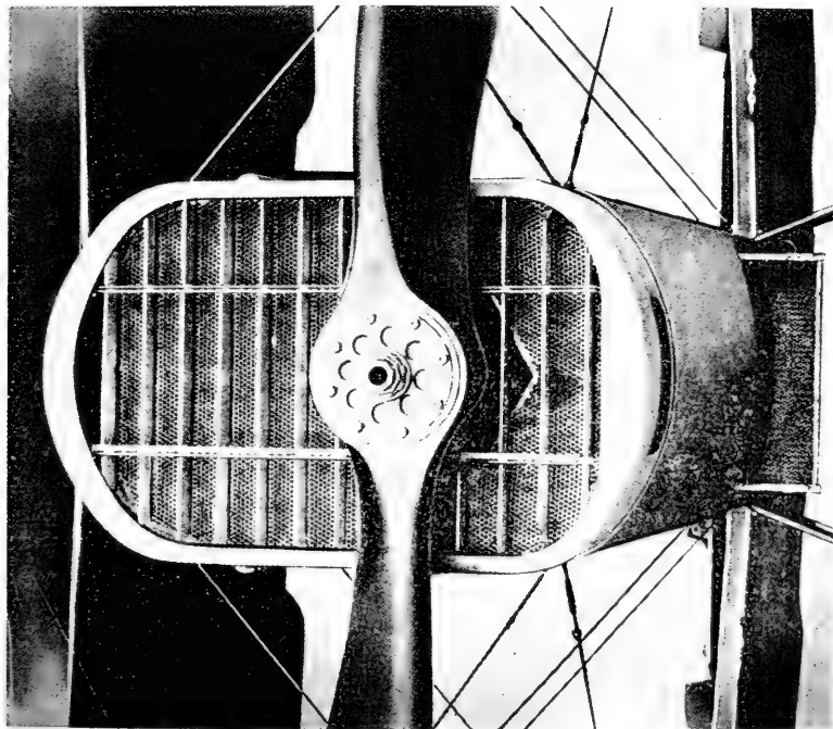
1. Large frontal coolant radiator for Liberty engine on Dell-4 airplane, 1918.
