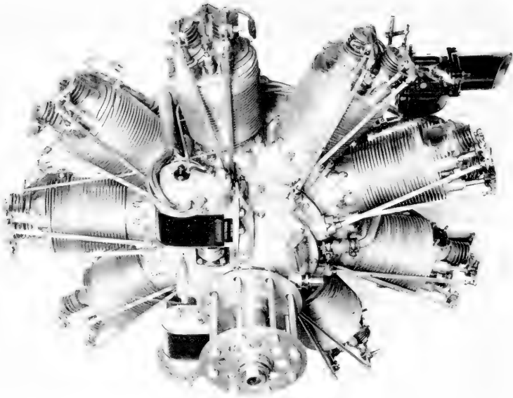
1. Lawrance J-1 air-cooled radial engine, 1924. The first American-designed 9-cylinder radial to be put into general use. The cast-aluminum cylinder head and internally-cooled exhaust valves have been retained in modern practice.
