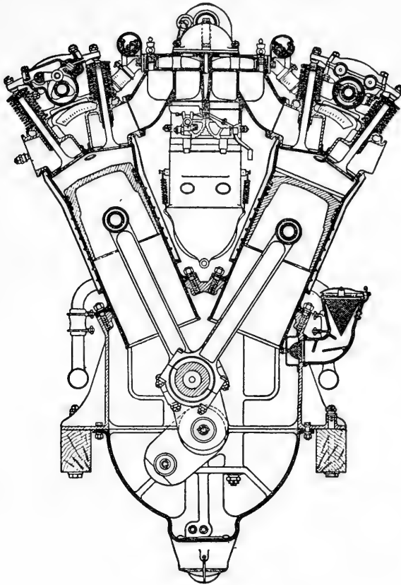
FIGURE 7.—“Liberty” engine, sectional transverse view.
