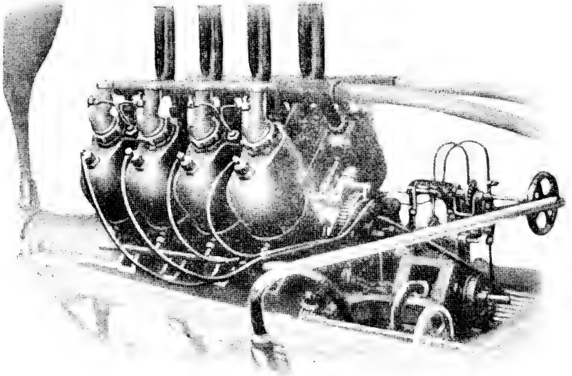
2. Antoinette engine, 8-cylinder, 55 hp.
