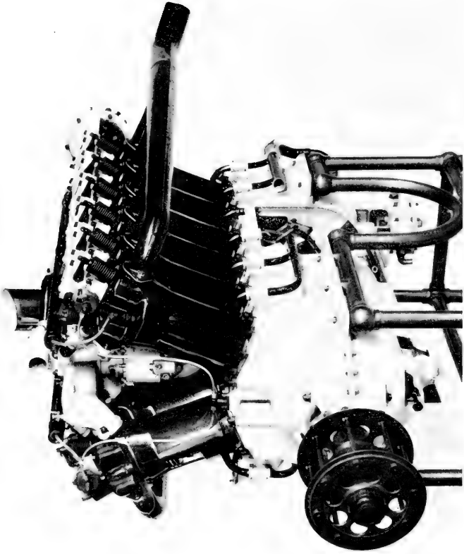
2. Liberty engine, 12-cylinder Vee, 400 hp., U.S.A., World War I.
