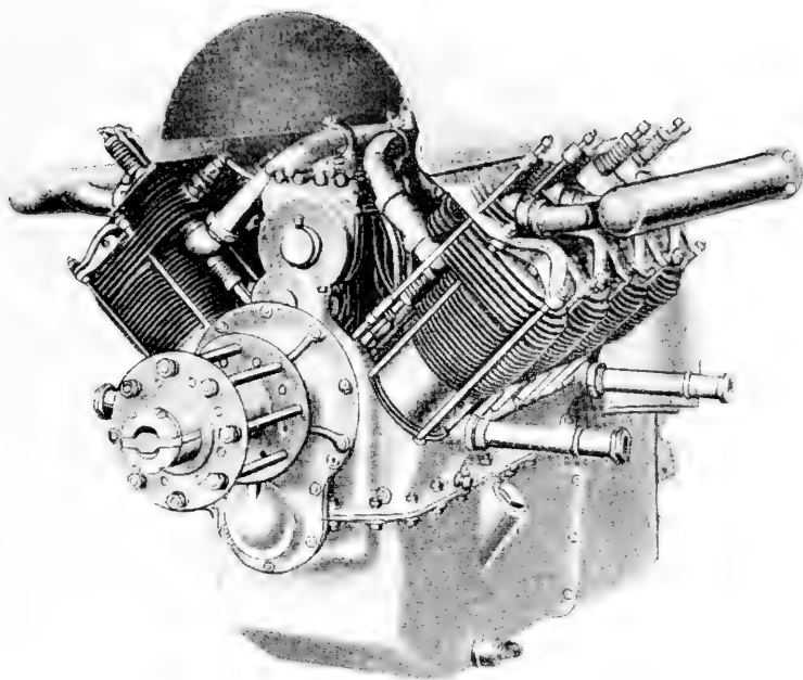
1. Renault engine, V-8, 80 hp.
