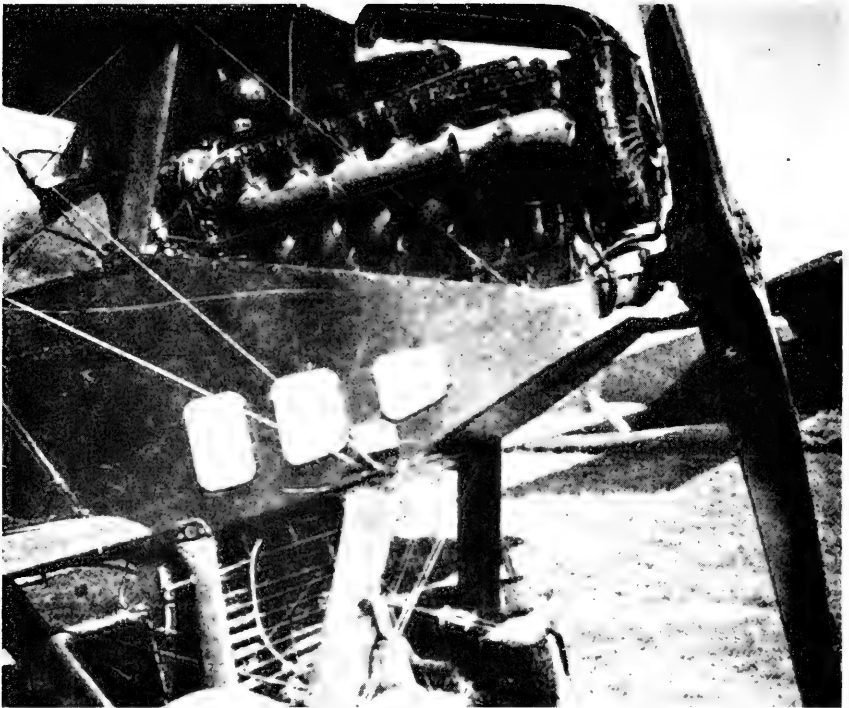
1. General Electric turbo-supercharger on Liberty engine, installed in LePere airplane which held the world altitude record for 1920, 1921, 1922.
