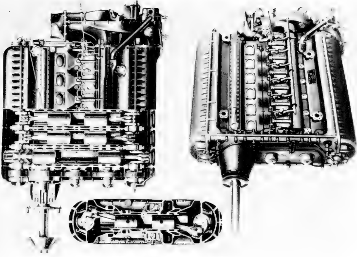
2. Junkers diesel engine.
