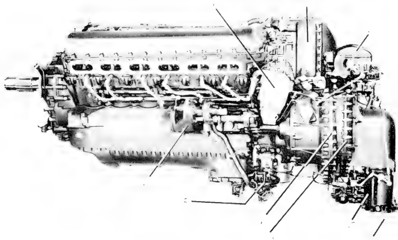
2. Rolls-Royce Merlin XX, 1944. 1, Left magneto; 2, aftercooler; 3, control unit; 4, carburetor air intake; 5, carburetor; 6, supercharger, first stage; 7, supercharger, second stage; 8, engine coolant pump; 9, aftercooler coolant pump.
