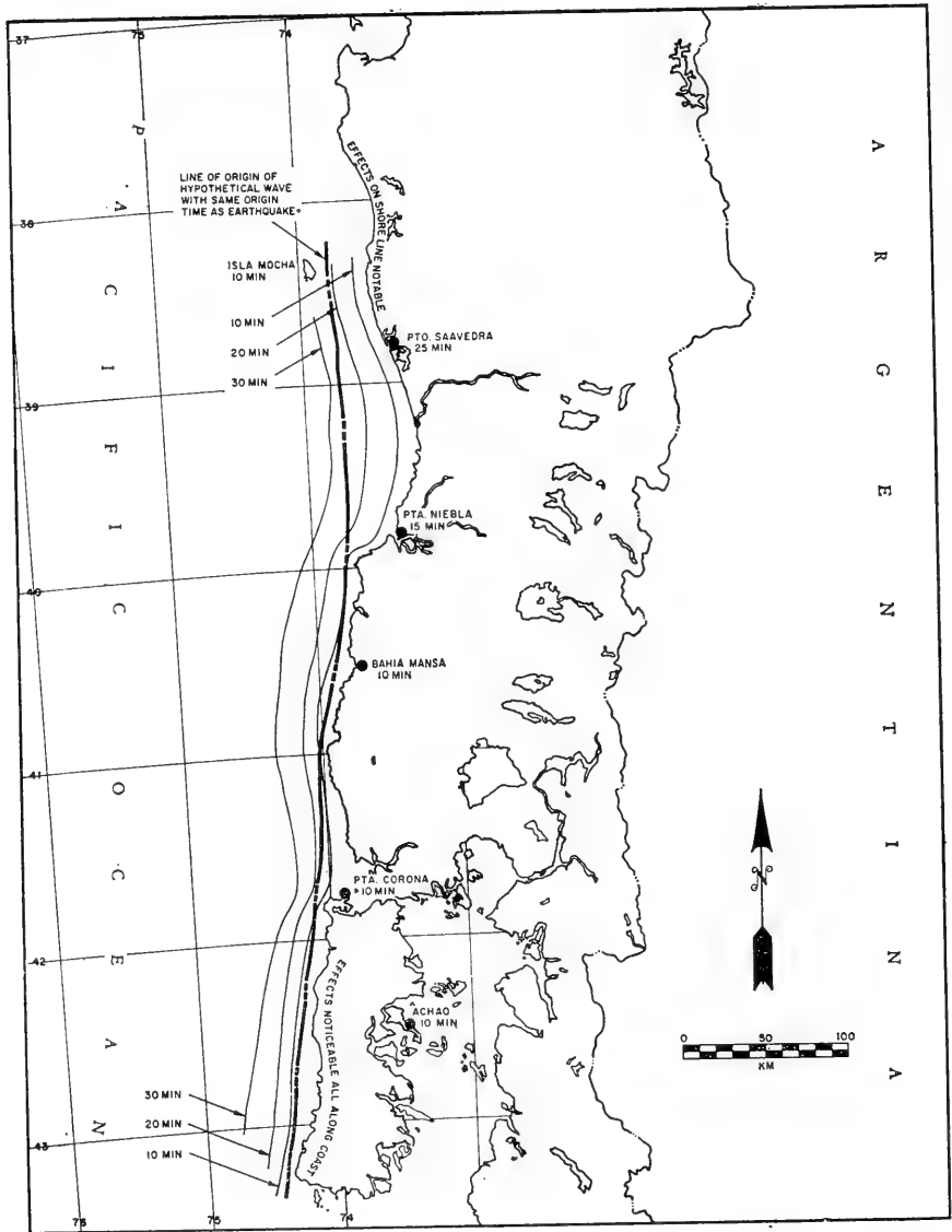
FIGURE 6.—Distance from shore that a wave can travel in indicated times, and estimated position of Maremoto if it began at the same instant as the earthquake.
