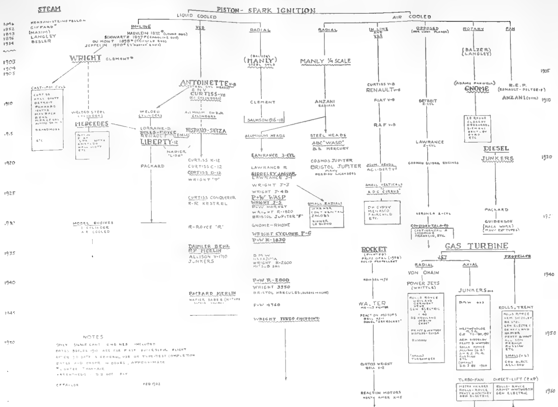
FIGURE 21 — The aircraft-engine family.
