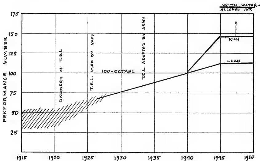
FIGURE 15.—Aviation fuel performance chart.
