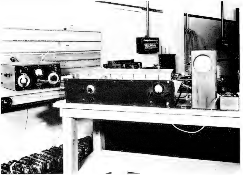
1. Original 28-Mc receiver with indicator on test bench showing (left to right) standard signal generator, receiver, indicator, audio output meter. 1936.
