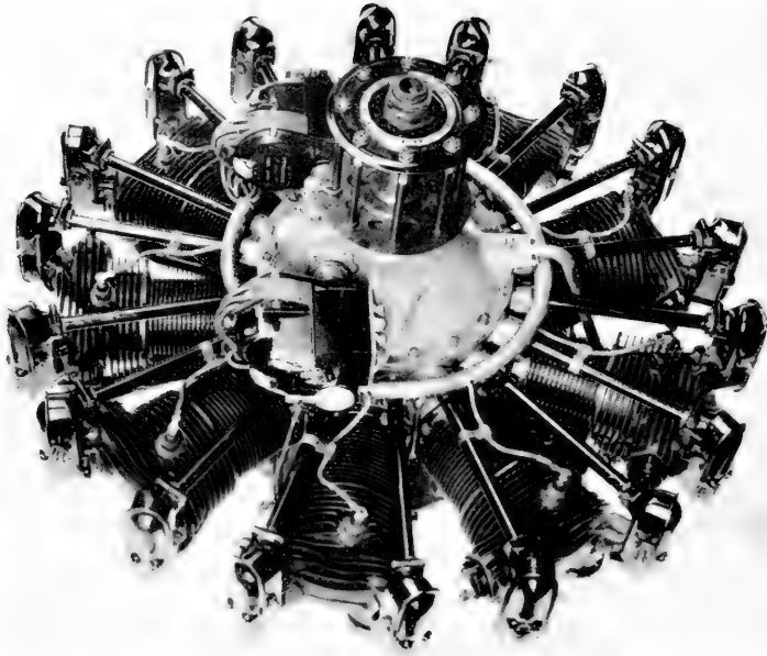
2. Wright Whirlwind engine of 1927. This type of engine was used by Lindbergh, Chamberlin, Byrd, and others.
