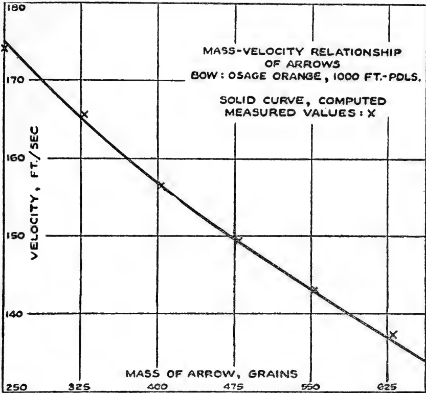
FIGURE 9.—Relation between mass of an arrow and its velocity when shot from a bow having 1,000 foot-pounds of available energy at full draw.
