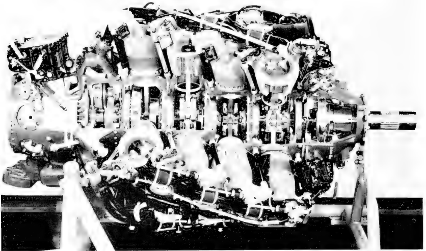
2. Pratt & Whitney R-4360, 28-cyl., 4-row air-cooled radial engine, 3350 hp., 1948, cutaway.
