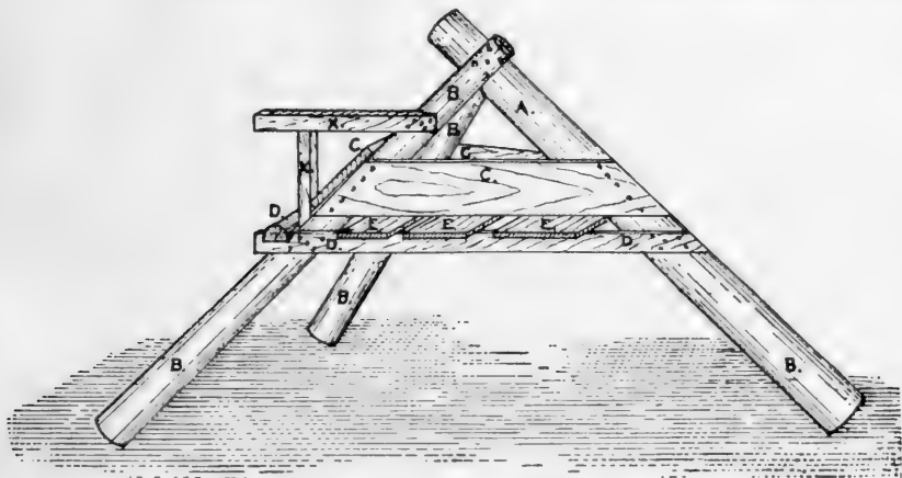
FIG. 1.—Three-legged rack horse or trestle: A.A. , horse head; B.B. , horse legs; C.C.C. , 12-inch boards to make sides of crib and also to act as braces; D.D.D. , leg braces which also support bottom of crib; E.E.E. , bottom of crib; X.X. , bracket for supporting walk.
