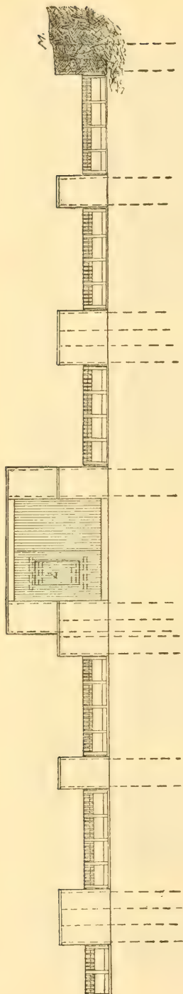
FIG. 3.—Front elevation of barrage shown in figure 2.
