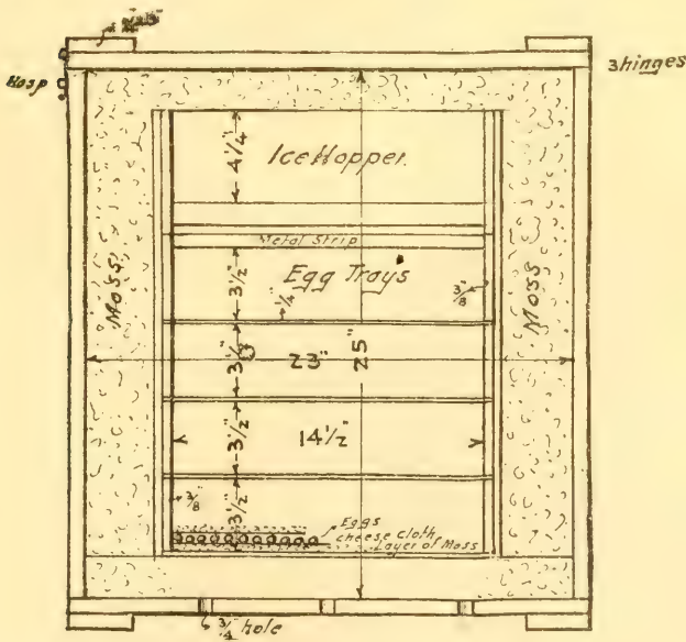
FIG. 9.—Atkins-Dinsmore shipping case. Cross section.
