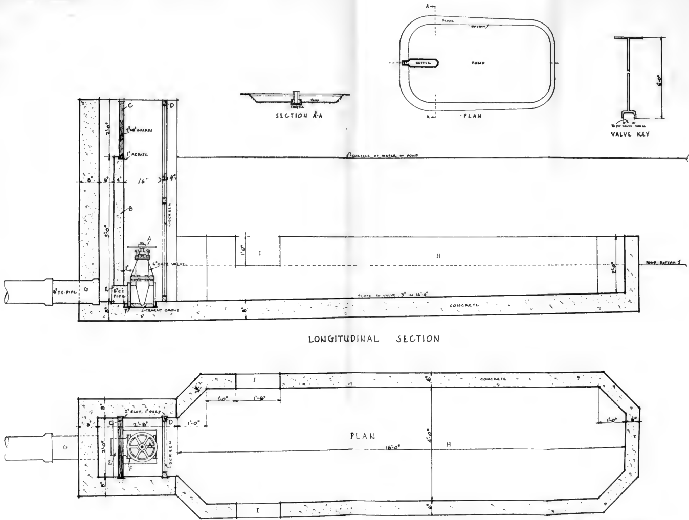
FIG. 3.—Plan of pond outlet and kettle for 68 ponds. (Designed by G. C. Leach.)
