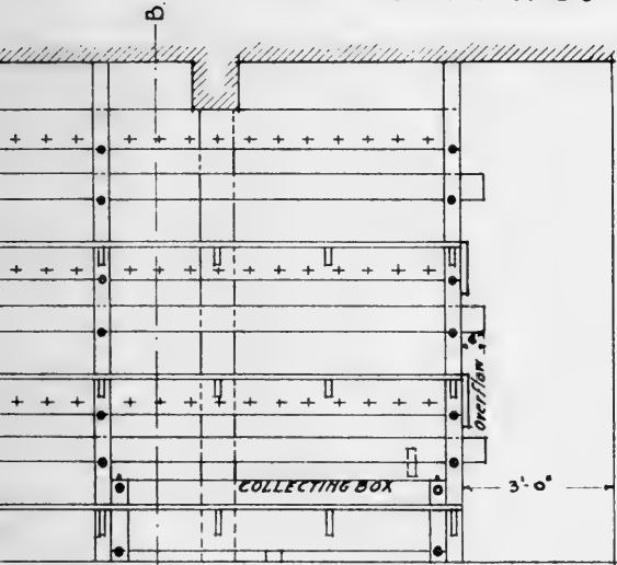
LONGITUDINAL SECTION AT JOINT BETWEEN SUPPLY & DRAIN TROUGH.
