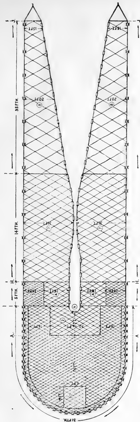
FIG. 3.—Lampara net. Section 1, 26-6 thread, \frac{1}{2} -inch mesh; 2, Mendocino or key of net 6-ply 3-inch mesh; 3, heavy netting, 6-ply, 1-inch mesh, 8 by 8 feet; 4, 6-ply, 3-inch mesh; 5, part of bag of 26-6 thread, \frac{1}{2} -inch mesh; 6, horseshoe, where wings divide; 7, wing-section of 5-inch mesh; 8, wing-section of 8 \frac{1}{2} -inch mesh; 9, strip of netting 10 inches wide, 16-ply, 1-inch mesh of heavy mesh, to hold bag to cork line and withstand wear and tear; H-H, cork line of \frac{3}{8} -inch diameter hemp rope, 300 corks in pairs, 6-inch interspace between pairs; H-J, wing cork lines, 500 corks in pairs on each wing, interspaces about 3 feet.
