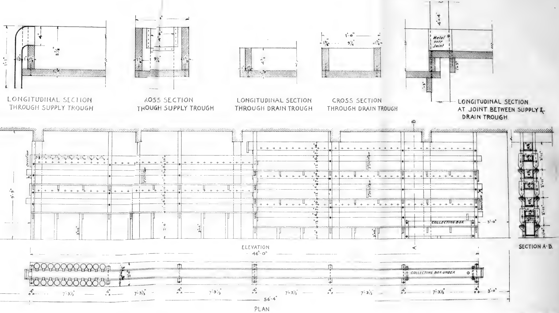
FIG. 1. Plan of hatching battery in use at the Cape Vincent (N. Y.) station for the incubation of whitefish and cisco eggs. (Designed by J. P. Snyder.)
