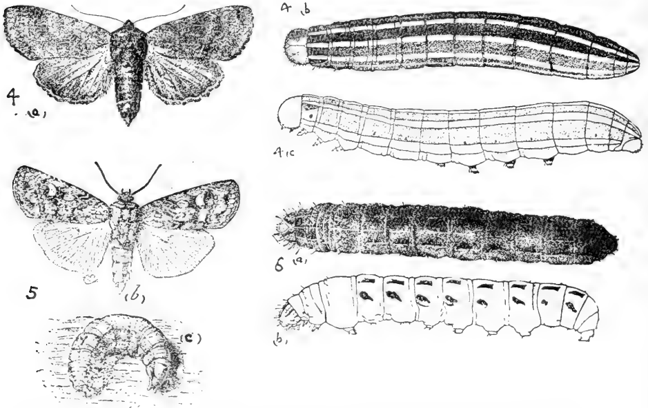
Cutworms : 4 (a) Nepheodes minians (Bronzed Cutworm) moth ; 4 (b) and 4 (c) larva or cutworm. 5 (b) Euxoa messoria (Dark-sided Cutworm) moth ; 5 (c) cutworm or larva. 6 Noctua clandestina (the W-marked Cutworm) larva.
