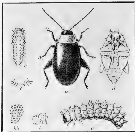
Spinach Flea-beetle : a , adult beetle ; b , egg mass ; bb , sculpture of egg ; c , full grown grub ; d , pupa ; e , newly hatched grub ; f , abdominal segment of same ; a, c, d , five times natural size ; b, e , more enlarged ; bb, f , still more enlarged. (After Chittenden, Bull. 19, N.S., Div. of Ent., U.S. Dept. Agr)
