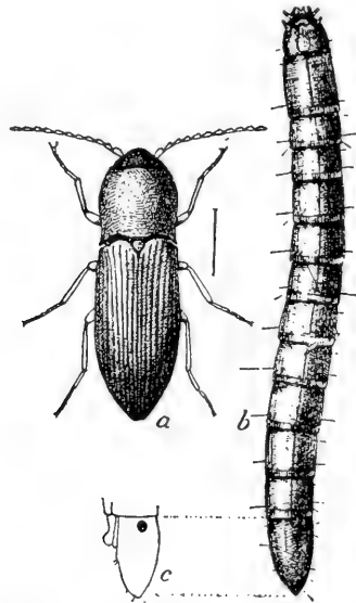
Agriotes mancus (Wheat Wireworm); A. adult beetle; B. wireworm or larva; C. last segment of larva.
