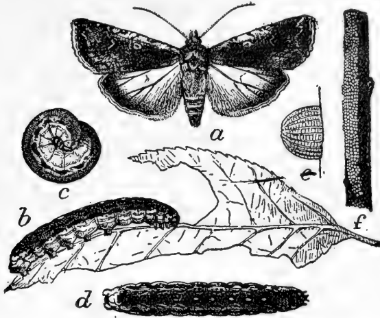
Peridroma Saucia. a, adult; b, c, d, full grown larve; e, f, eggs. All natural size except e, which is greatly enlarged. (From Yearbook U. S. Dept. Agric. 1898.) Life-history of a cutworm.
