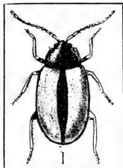
Horse Radish Flea beetle, enlarged 9 times. (After Chittenden, Insect Life, Vol. VII.)
