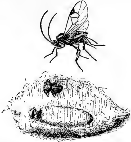
Apanteles lacticolor , adult female and cocoon. A parasite of the Brown-tail Moth, much enlarged. (Bull. 91, U.S. Dep. Agric.)
