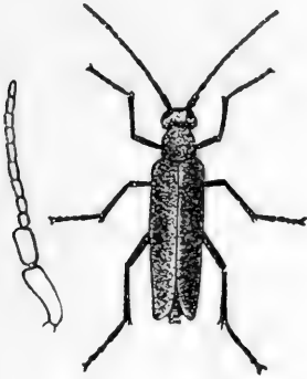
Ash-Gray Blister Beetle
